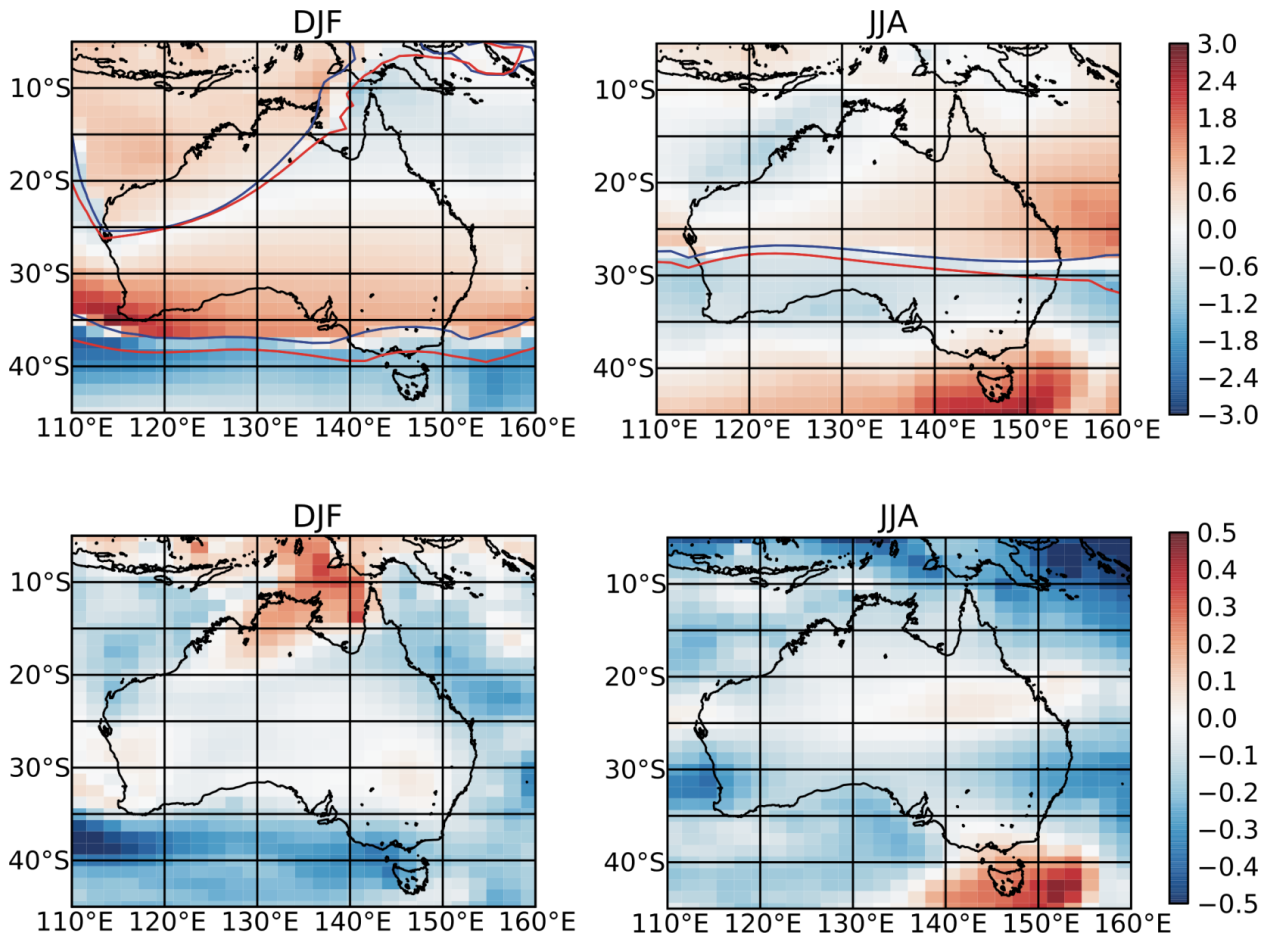
Figure 10: Top: CC-A modelled changes in wind speed for DJF and JJA with zero of zonal wind speed shown as a contour in blue for current climate and red for future climate. Bottom: standard deviation of wind speed for DJF and JJA as modelled by CC-A.
