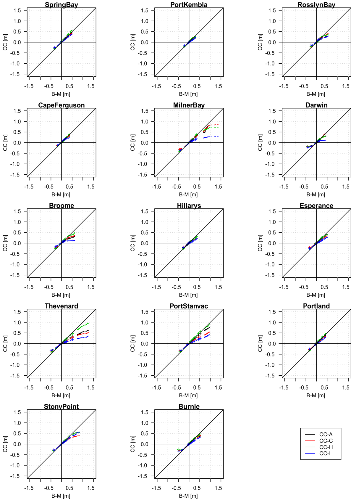
Figure 7: Q-Q plots comparing the sea levels from the four 1980-1999 CC simulations versus the B-M simulation. Note that for clarity only the '+' symbols are used to denote the 0.1, 1, 10, 50, 90, 99, and 99.9th percentiles.
