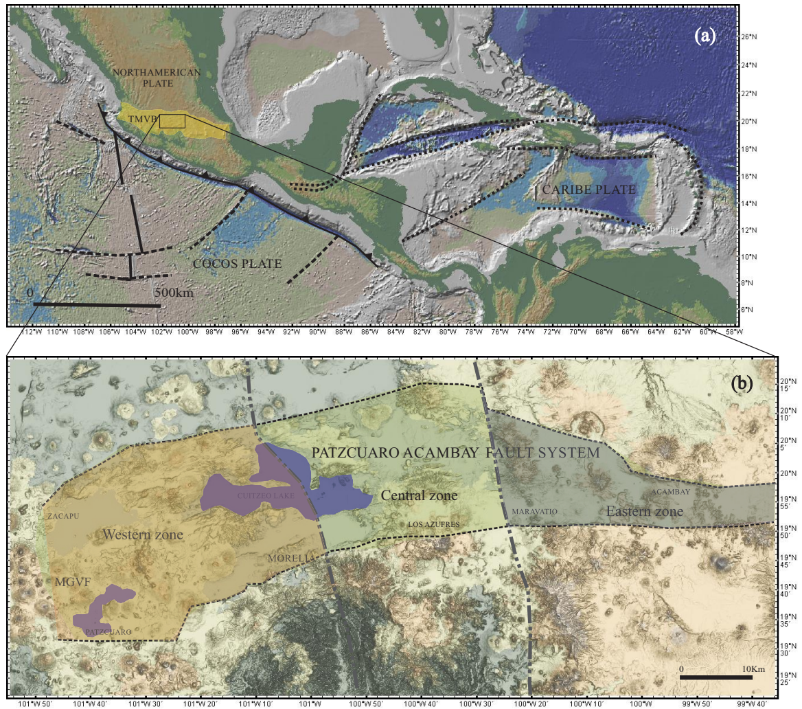
Figure 1. (a) Tectonics and geodynamic setting of the Trans-Mexican Volcanic Belt (yellow area). Dotted black lines are plate boundaries and the continuous black line is the Middle America Trench. The Pátzcuaro-Acambay Fault System (PAFS) is outlined by the black rectangle. TMVB: Trans-Mexican Volcanic Belt. (b) Tectonic area of the Pátzcuaro-Acambay Fault System that shows the limits (thick dashed gray lines) between the three zones of the PAFS (western, central and eastern zones). MGVF: Michoacán-Guanajuato Volcanic Field.
