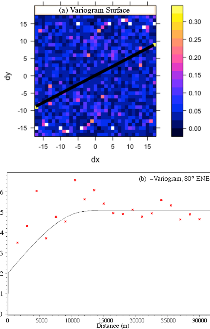
Figure 5. (a) Variogram surface of fault lengths in the PAFS, with a straight line showing the direction of the best spatial autocorrelation. At the center a pattern forms a shape of an ellipse, suggesting that the best correlations are observed in NE-SW direction. (b) Anisotropic variogram of fault lengths, which exhibits a good structure in ENE direction ( 80^\circ ), and matches with a spherical model (black continuous line). So, this faults are optimally oriented in relation to the current stress in the PAFS ( \sigma_2 ). So, this anisotropic direction indicates that the spatial distribution of faults is mainly due to extensional stresses, and is consequently subject to deformation generated by the current stress field in the PAFS ( \sigma_2 , NW-SE).
