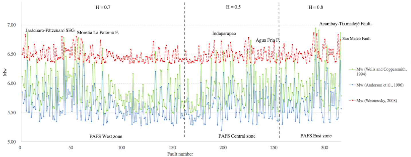
Figure 3. Firmagram roughness graph for the earthquake magnitude variations calculated by the surface rupture length (SRL) for the PAFS using: Wesnousky (2008, data in red); Wells and Coppersmith (1994, data in green) and Anderson et al. (1996, data in blue). By optical visualization we observed that Wells and Coppersmith (1994) and Anderson et al. (1996) are underestimating the data with respect to the magnitudes determined by the equivalent regression model proposed by Wesnousky (2008). Dashed gray lines are delimiting the three zones that define the micro-regionalization of the PAFS (western PAFS , central PAFS and eastern PAFS ) in terms of their Hurst exponent ( H_w = 0.7, H_w = 0.5, H_w = 0.8 respectively), showing different seismic rates for each zone. Some fault names were printed in the figure.
