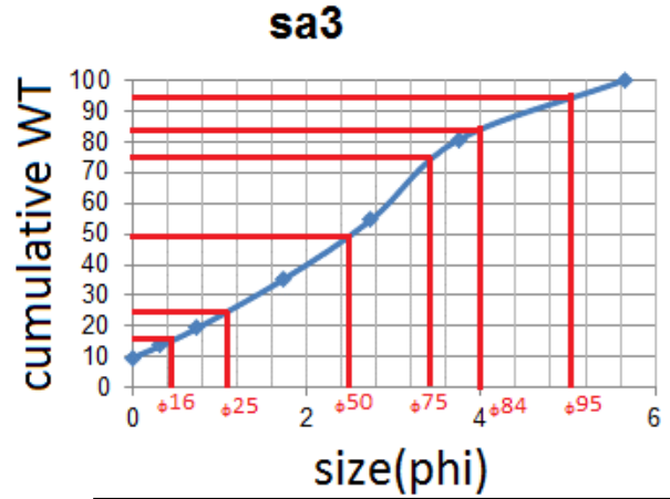
Fig.S18-3 cumulative weight with grain size in Phi unit of core 3 sample no. 3
