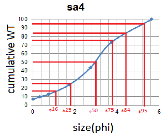
Fig.S16-4 cumulative weight with grain size in Phi unit of core 1 sample no. 4
