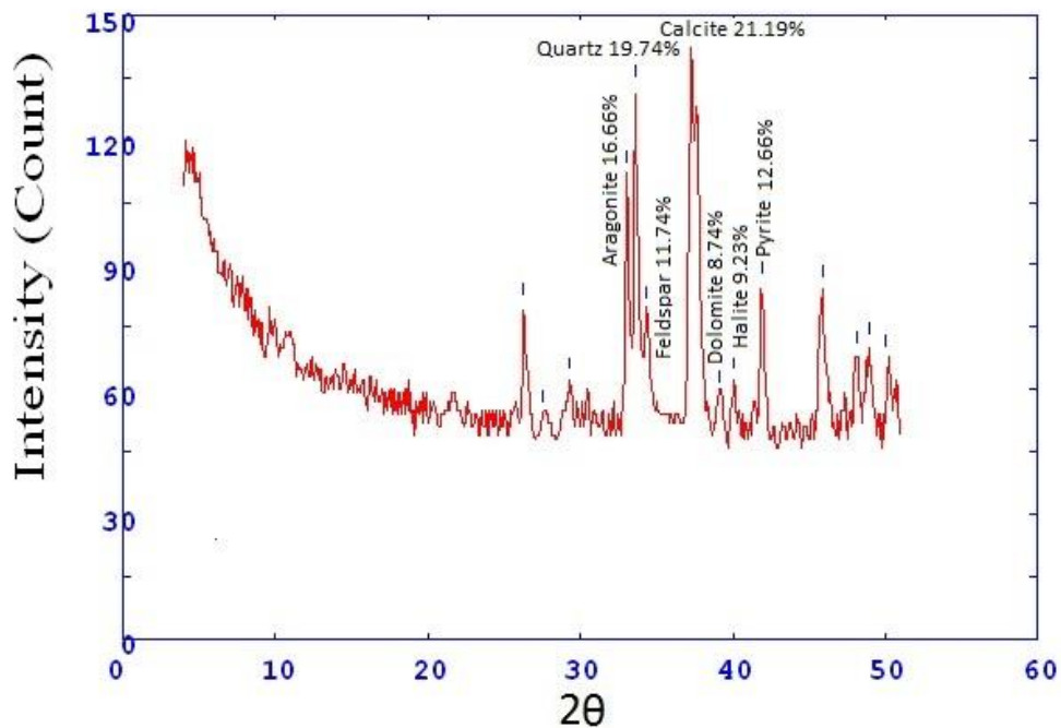
Fig.S11-8 X ray diffractogram of core 8 sample no.8
