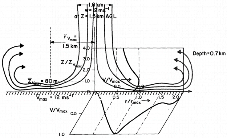
Figure 2: Scheme of a thunderstorm downburst and nose velocity profile in the radial outflow (After Hjempfelt 1988).
