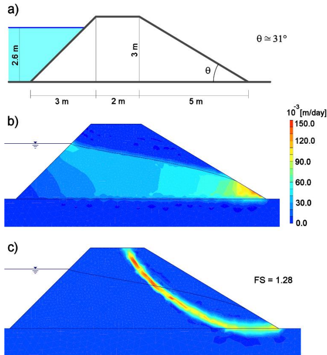
Figure 7: - a) cross sectional sketch of a stable dam with the main elements dimension; b) water velocity field moving in the dam body and associated phreatic surface; c) failure surface generated by a factor of safety of 1.28.
