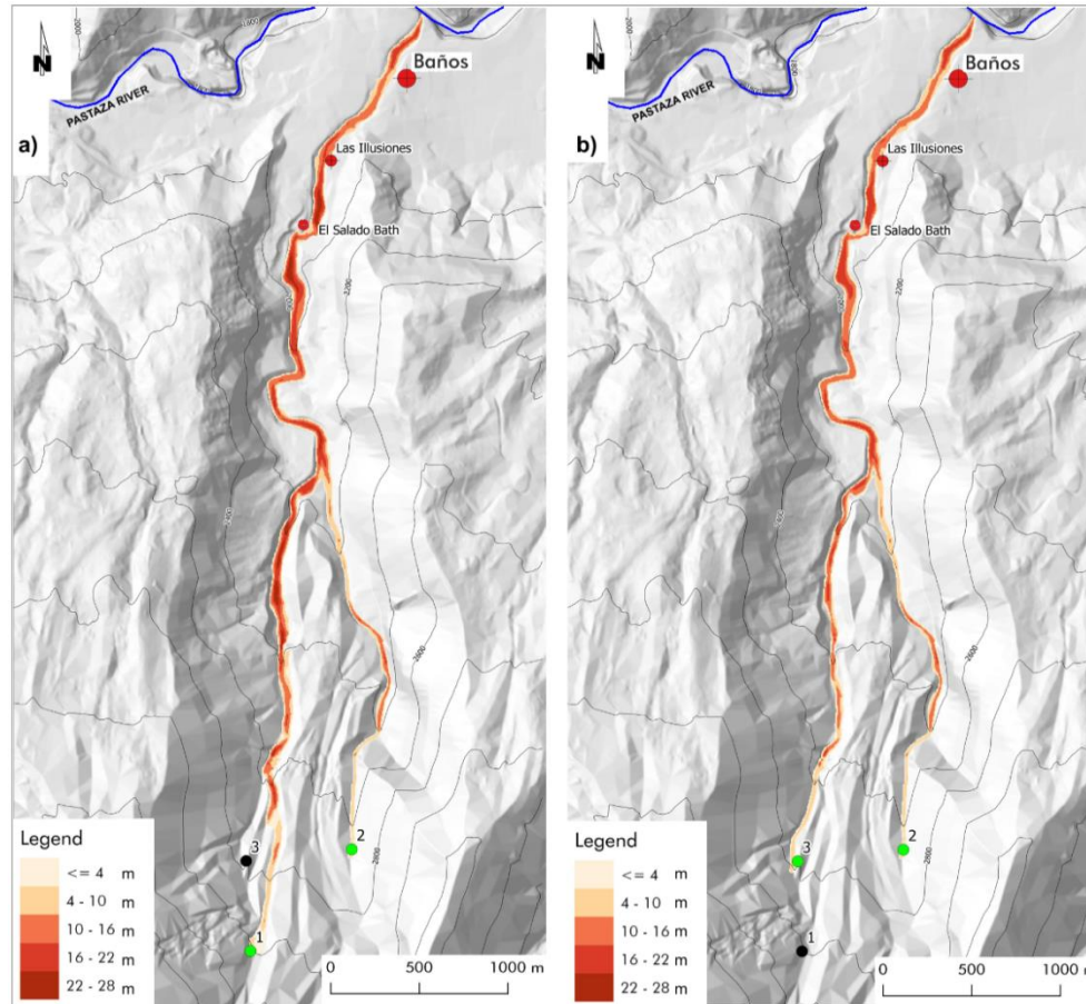
Figure 9: Simultaneous triggering of lahars from points 1 and 2 (a), from points 2 and 3 (b). The maximum thickness of the lahar during the conjectured events is reported in meters according the legend.
