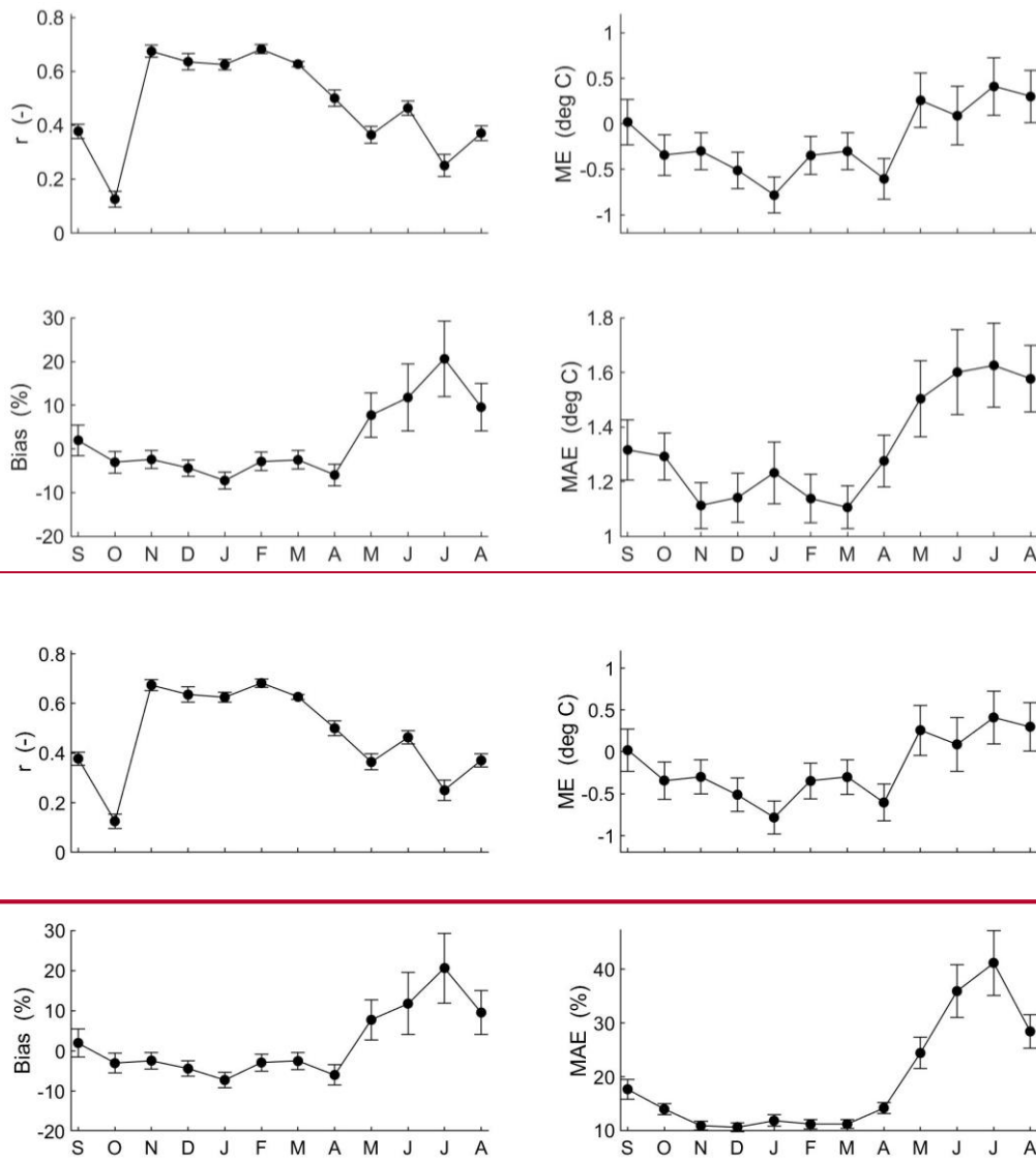
Fig. 4. Same as Fig. 3 but for accuracy measures of satellite-based gridded air temperature data product.
