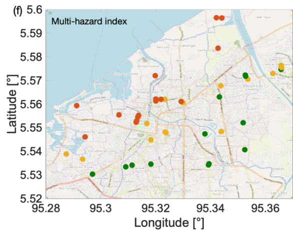
Figure 8 Application to the seismic and tsunami indices to 85 RC school buildings in Banda Aceh, Indonesia.
