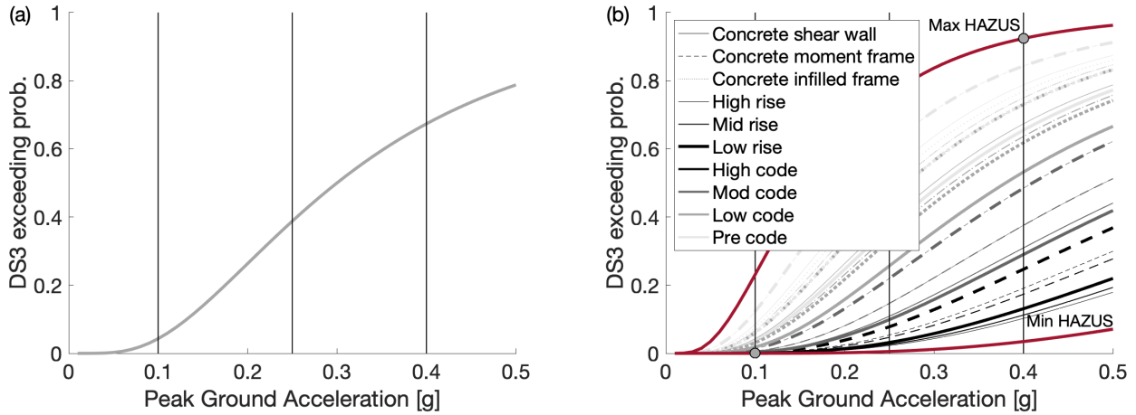
10 Figure 2 a) Example baseline score for a given archetype building typology. b) HAZUS fragility curve database related to the Extensive Damage limit state for RC buildings.
