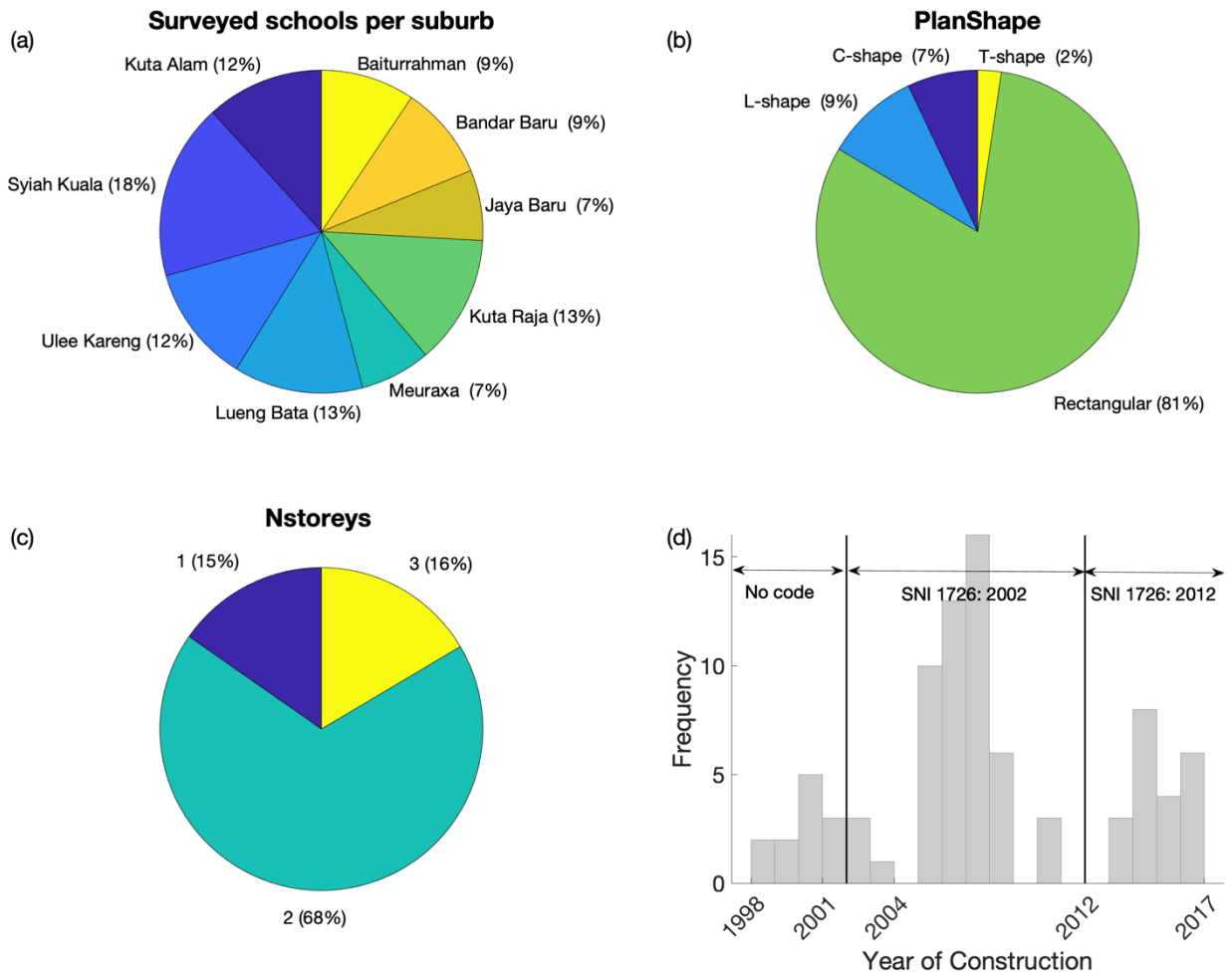
5 Figure 6 Statistics for the 85 surveyed school buildings.
