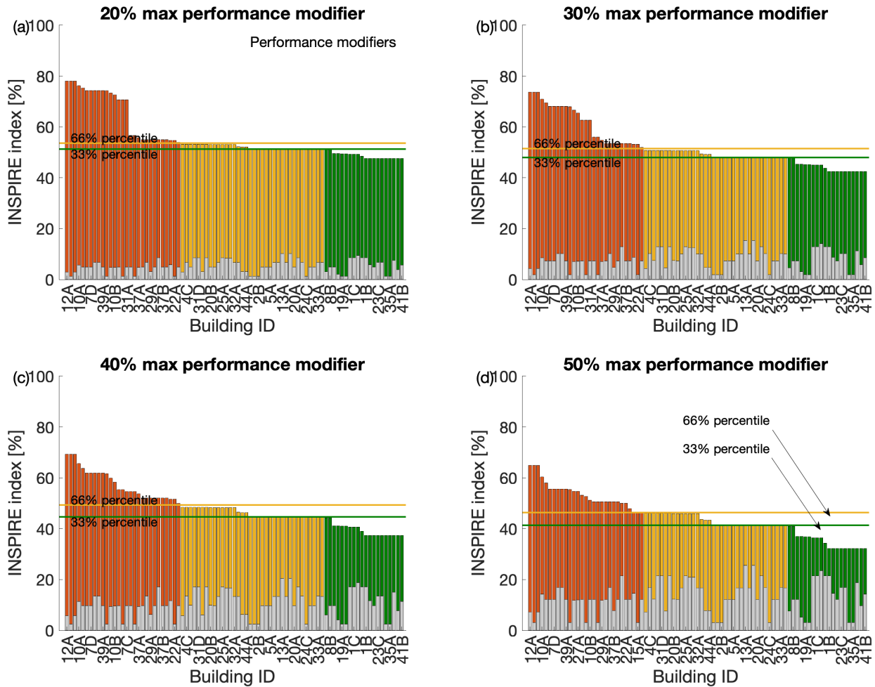
Figure 9 Sensitivity analysis for the baseline-to-performance modifier ratio.
