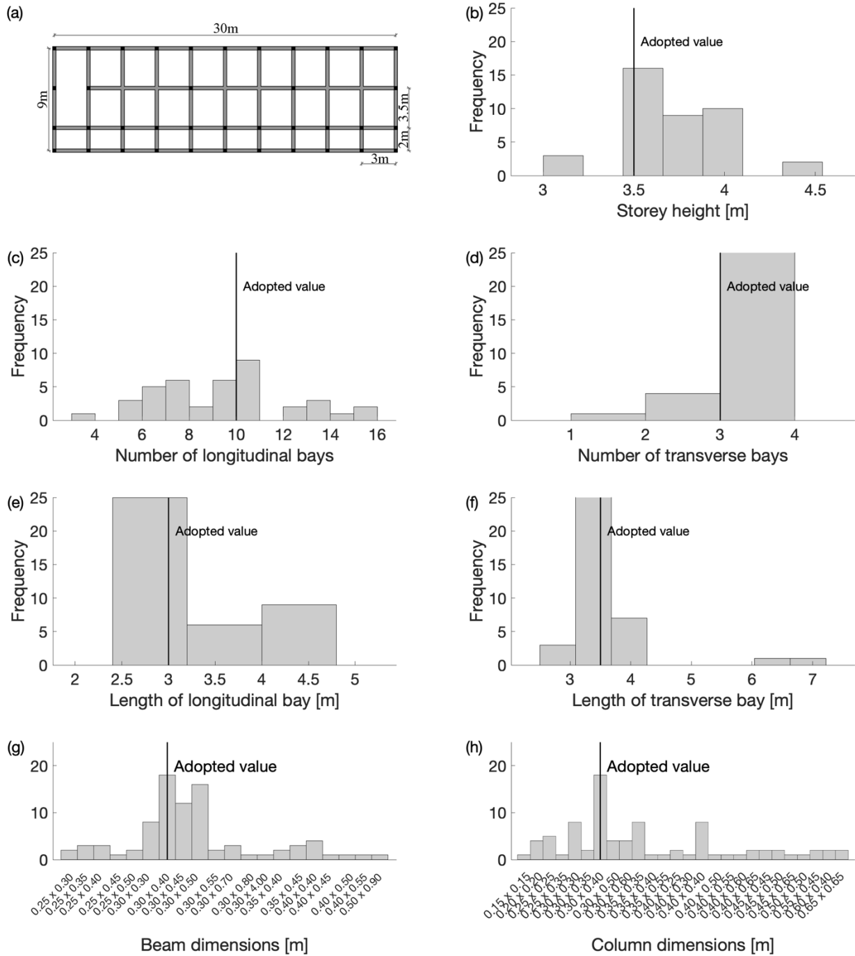
Figure 7 shows the geometrical characteristics of the archetype building geometry, which are based on the modal (most frequent) values of the empirical distributions (histograms) considering only the rectangular, 2-storey buildings in the portfolio
