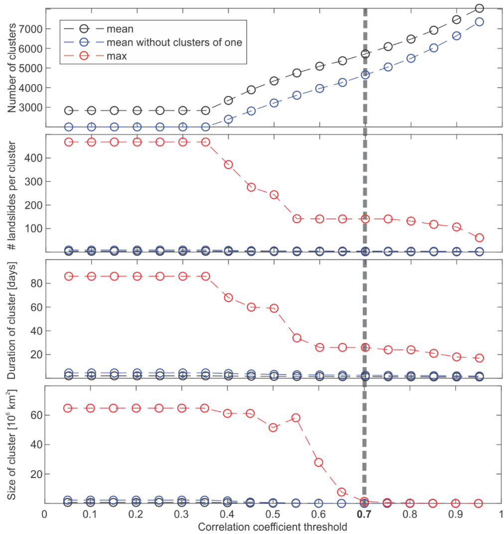
Figure S1. Impact of the chosen threshold for the spearman correlation coefficient on total number of clusters in the global landslide catalog, on the average number of landslides per cluster, on the average duration of landslide clusters, and on the average area of landslide clusters. In this study a threshold of 0.7 was chosen as from this point onwards maximums size of, duration of and landslides per cluster, becomes stable compared to the original values.
