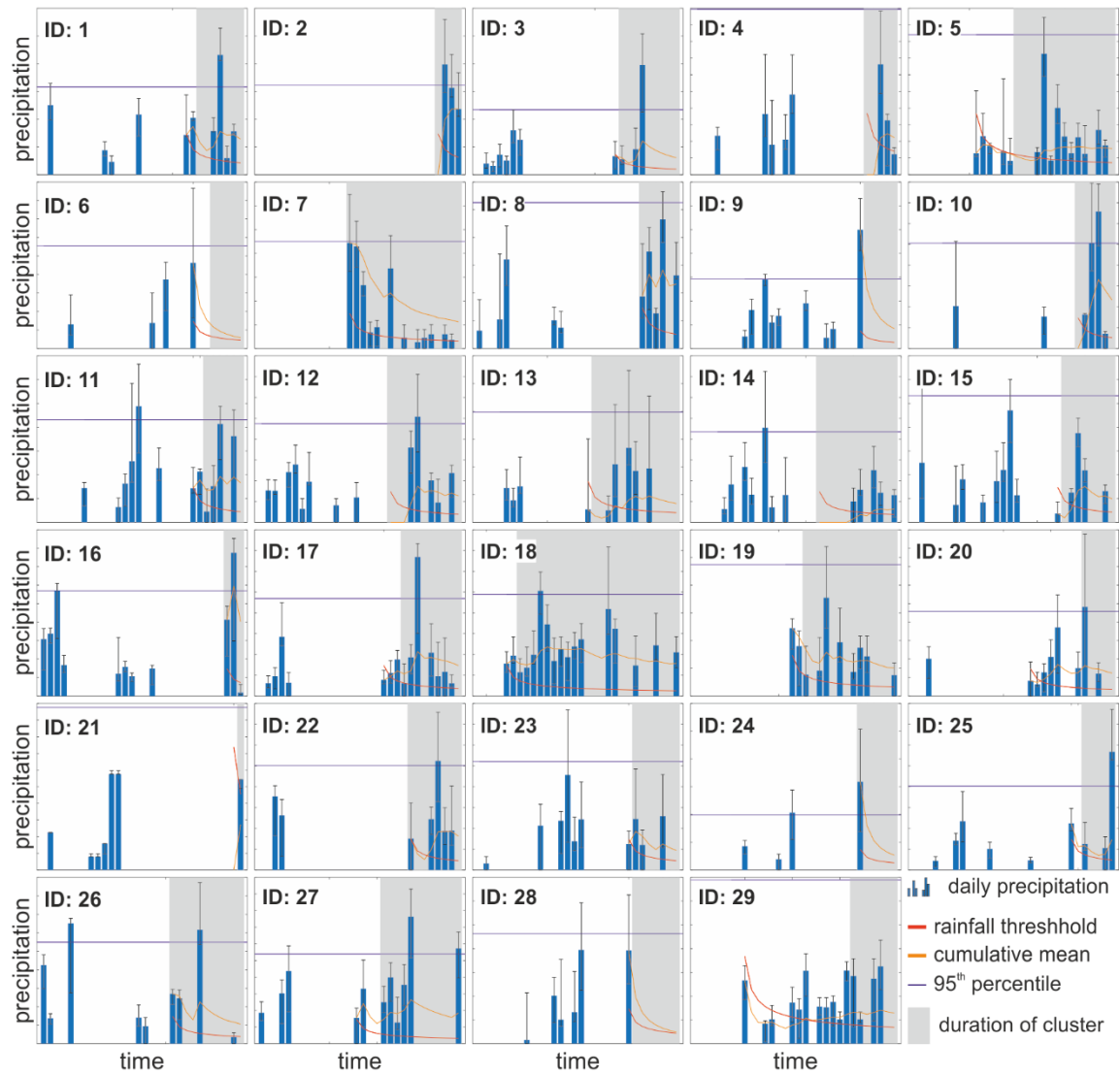
Figure S3. Median Rainfall (error bars show inner quartile range) in the 30 days preceding the last landslide event of the clusters located in the West Coast of North America. The blue line indicates the 95 th percentile of rainfall (excluding rain-free days). Given in red is the global rainfall threshold (ID from Guzzetti et al. 2008) and in orange the cumulative mean for the rainfall event preceding the cluster.
