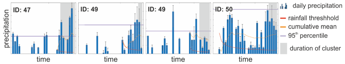
Figure S7. Rainfall in the 30 days preceding the last landslide event of the clusters located in the Philippines. The blue line indicates the 95 th percentile of rainfall (excluding rain-free days). Given in red is the global rainfall threshold (ID from Guzzetti et al. 2008) and in orange the cumulative mean for the rainfall event preceding the cluster.
