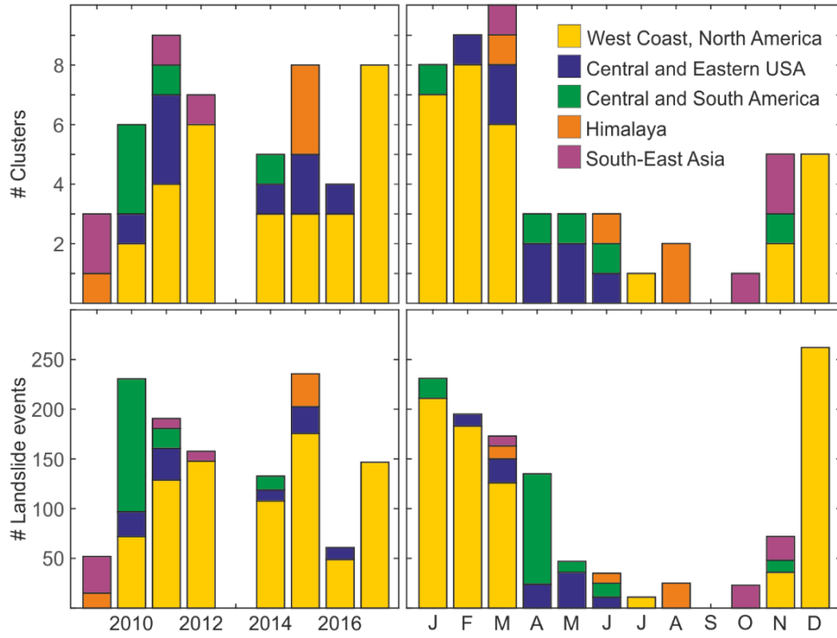
Figure S2. Recorded landslide clusters throughout the years and seasons for all of the 5 distinct regions.
