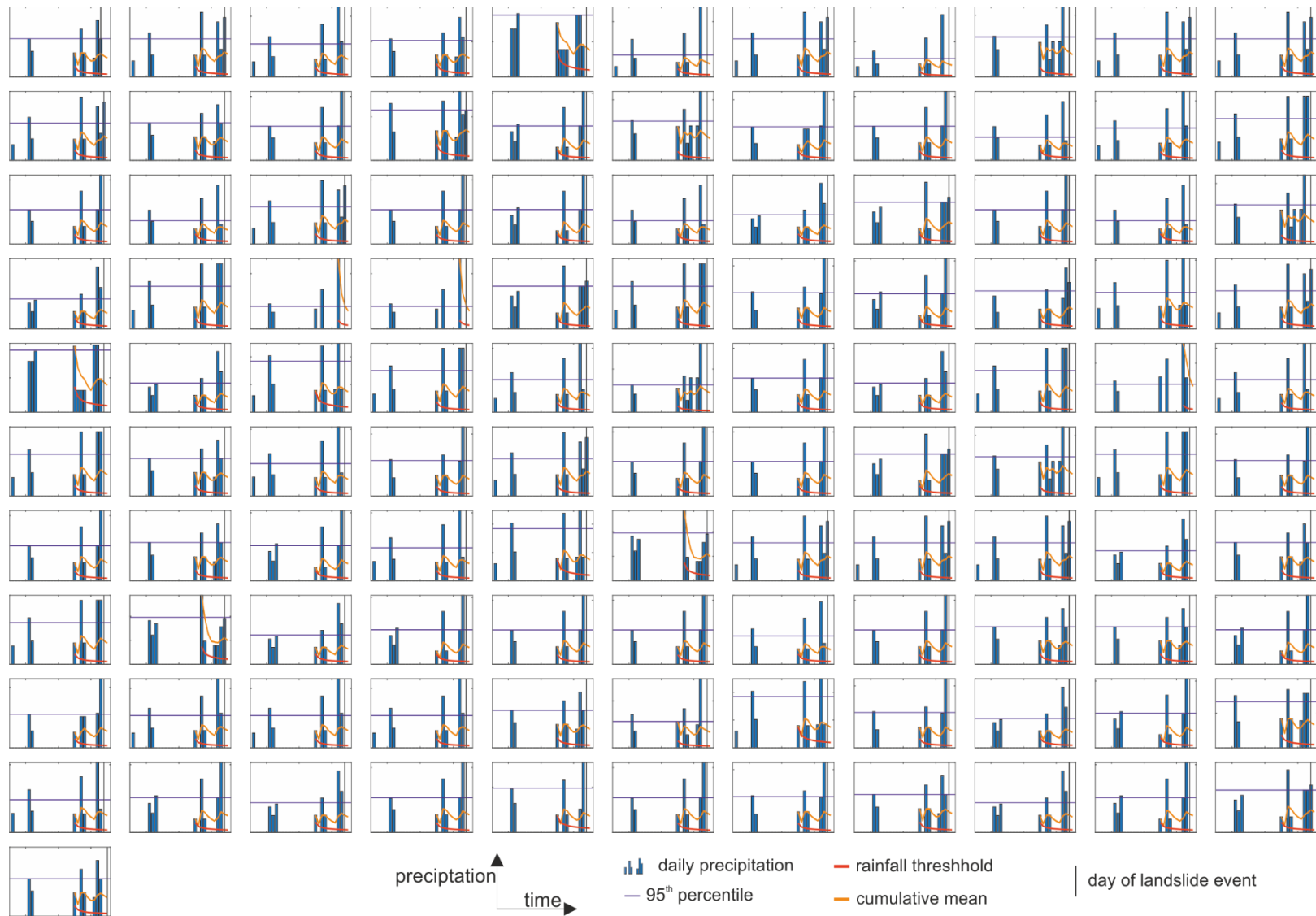
Figure S8. Rainfall at the location of all events associated with the cluster in Rio de Janeiro with the most events per day. Shown is daily precipitation of the 30 days preceding the last event of the cluster.
