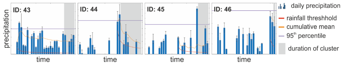
Figure S6. Rainfall in the 30 days preceding the last landslide event of the clusters located in the Himalaya Region. . The blue line indicates the 95 th percentile of rainfall (excluding rain-free days). Given in red is the global rainfall threshold (ID from Guzzetti et al. 2008) and in orange the cumulative mean for the rainfall event preceding the cluster.
