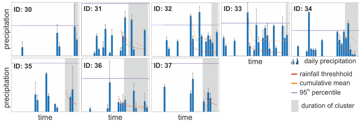
Figure S4. Rainfall in the 30 days preceding the last landslide event of the clusters located in Central and Eastern USA. The blue line indicates the 95 th percentile of rainfall (excluding rain-free days). Given in red is the global rainfall threshold (ID from Guzzetti et al. 2008) and in orange the cumulative mean for the rainfall event preceding the cluster.
