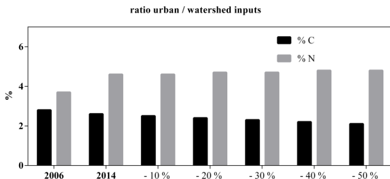
Figure 3: ratio of urban to watershed inputs of carbon and nitrogen in % for different scenarios.
