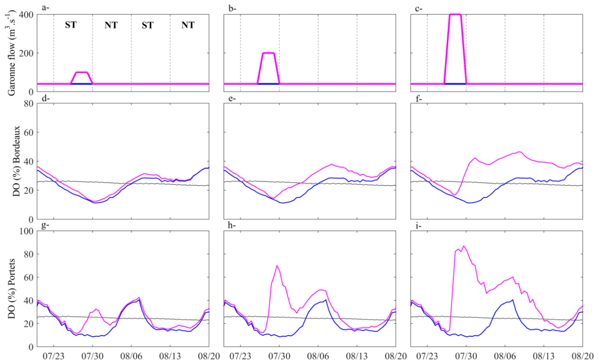
Figure 4: Time series of river flow (top, \text{m}^3\text{s}^{-1} ), \text{DO}_{\text{min}} (over tidal cycle) at Bordeaux (middle, %sat) and DO at Portets (bottom, %sat) for the scenarios of short river flow increases by 100 \text{ m}^3\text{s}^{-1} (a, d and g), 200 \text{ m}^3\text{s}^{-1} (b, e and h) and 400 \text{ m}^3\text{s}^{-1} (c, f and i). Blue line represents the simulation of reference.
