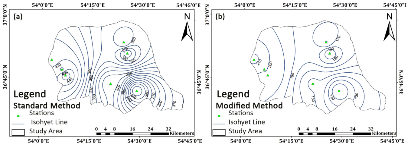
Figure 2: The spatial distribution of PMP 24 using (a) the standard and (b) the modified approaches in study area.
