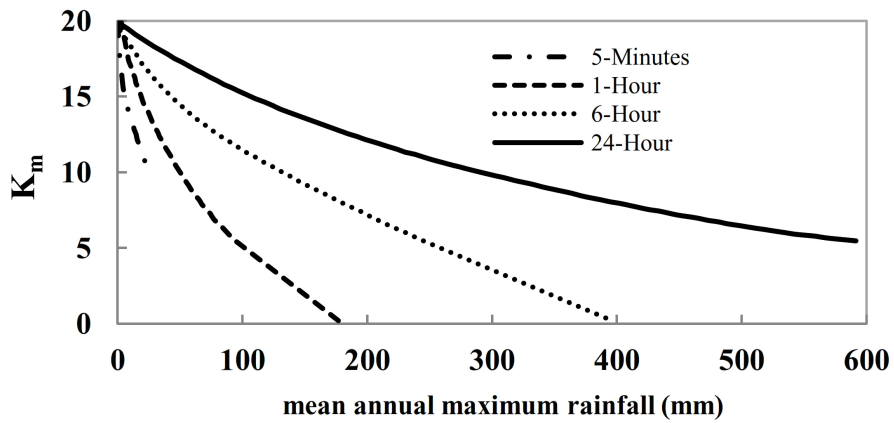
K m charts that were extracted by authors
