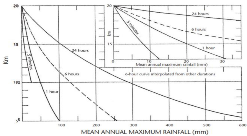
K m charts (WMO, 2009)
