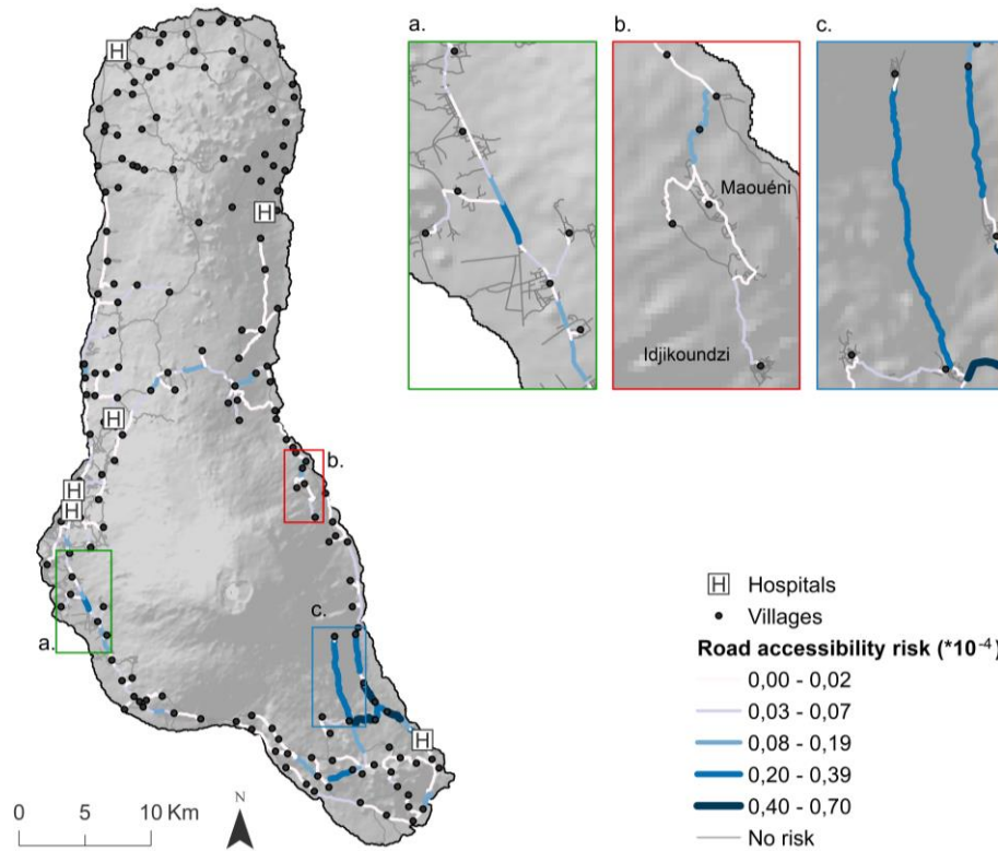
Figure 8 - Accessibility risk map for road segments combining road access vulnerability based on travel time (s) to the closest infrastructure with road segment susceptibility to lava flows.
