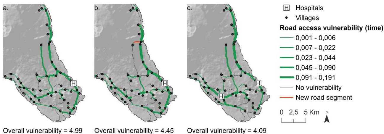
15 Figure 10 - Modification of the actual road access vulnerability (a) by constructing a new road segment (b) or by developing a new infrastructure (c). The overall road access vulnerability is the sum of the road access vulnerability values of all road segments within the Foubouni hospital service area.
