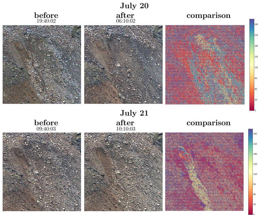
Figure 5. Close-up images (800 * 800 pixels) taken from the webcam during the internally-driven events of 20 th July and 21 st July 2017. First column shows the last exploitable image (with its exact timing) before the associated event, the second column the first exploitable image after the event. The third column shows the differences between the two images using a heatmap (arbitrary ranging between 0 and 256) where yellow and blue colors highlight locations experiencing the larger mismatch between images. These differences are evaluated for each pixel as the maximum of the absolute difference on each channel (red, green and blue) separately.
