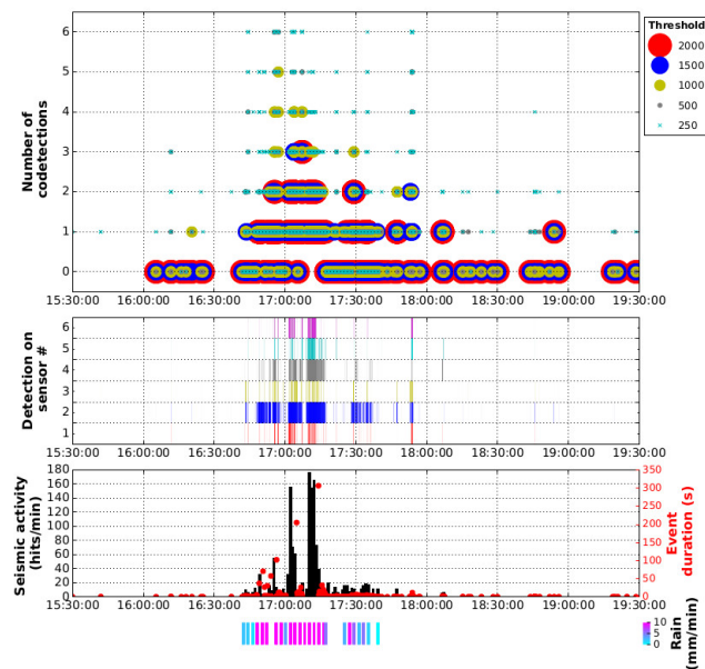
Figure 7. Externally-driven event (top panel: 10 July, bottom: 18 July): Number of co-detection using different thresholds, their associated detecting sensors (same arbitrary unit as in Fig. 4), the corresponding seismic activity (and event duration) and the precipitation record during this period.
