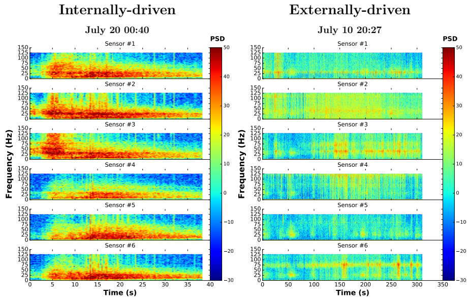
Figure 8. Typical power spectral densities (i.e. spectrograms) associated with internally and externally-driven events, plotted with the same scale. Frequency domains are colored from red for high power to blue for low power.
