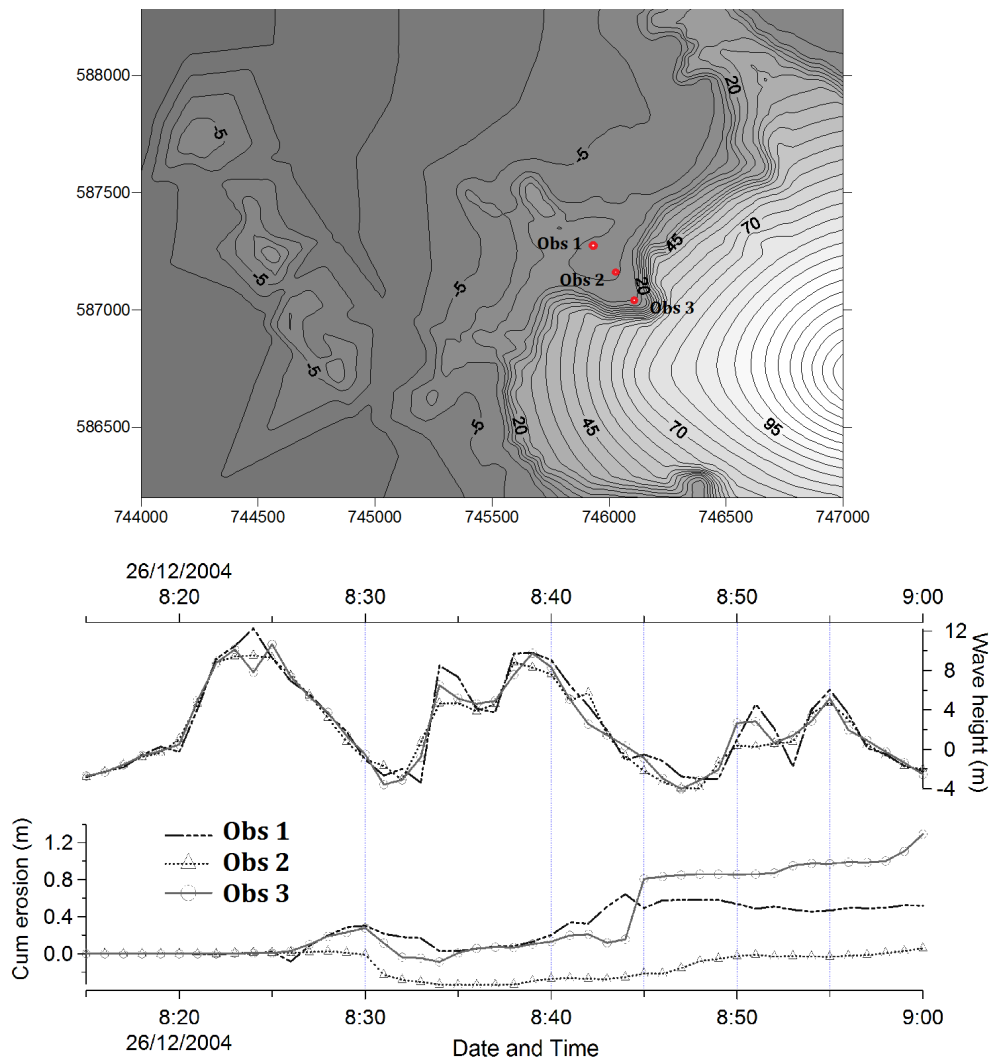
Figure 8: Correlation between wave height and cumulative sediment on the observation points.
