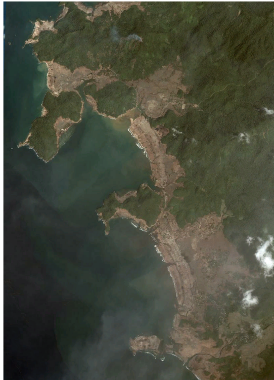
Fig. 1. Landsat satellite image captured on February 2nd, 2005 showing the tsunami inundation area (DigitalGlobe, 2019).
