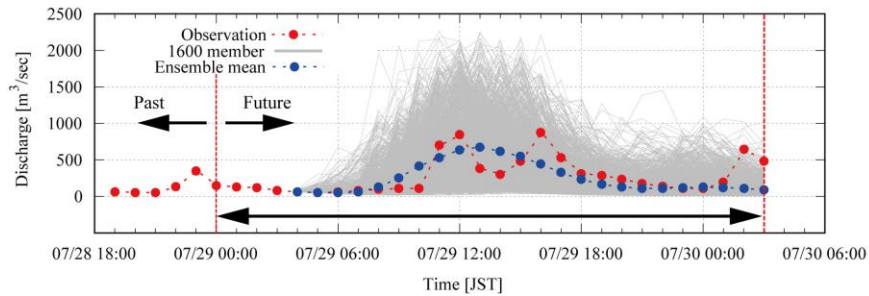
Figure 6. The hydrographs of (a) 11 discharge simulations in Part 1 (Kobayashi et al., 2016), (b) same 11 member but with a positional shift in Part 1, (c) 50 discharge simulations with 4D-EnVAR-NHM and (d) 1600 discharge simulations with 4D-EnVAR-NHM.
