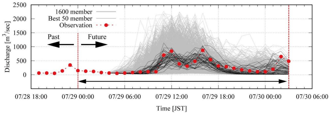
Figure 12. Hydrographs of all 1600 ensemble members, the 50 best ensemble members ( \text{NSE} > 0.224 ), and observations.
