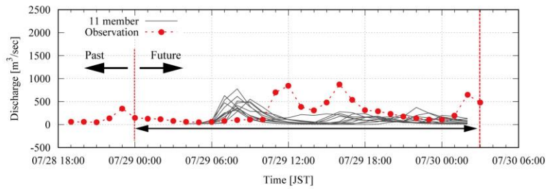
(b) 11 member (position shift)
