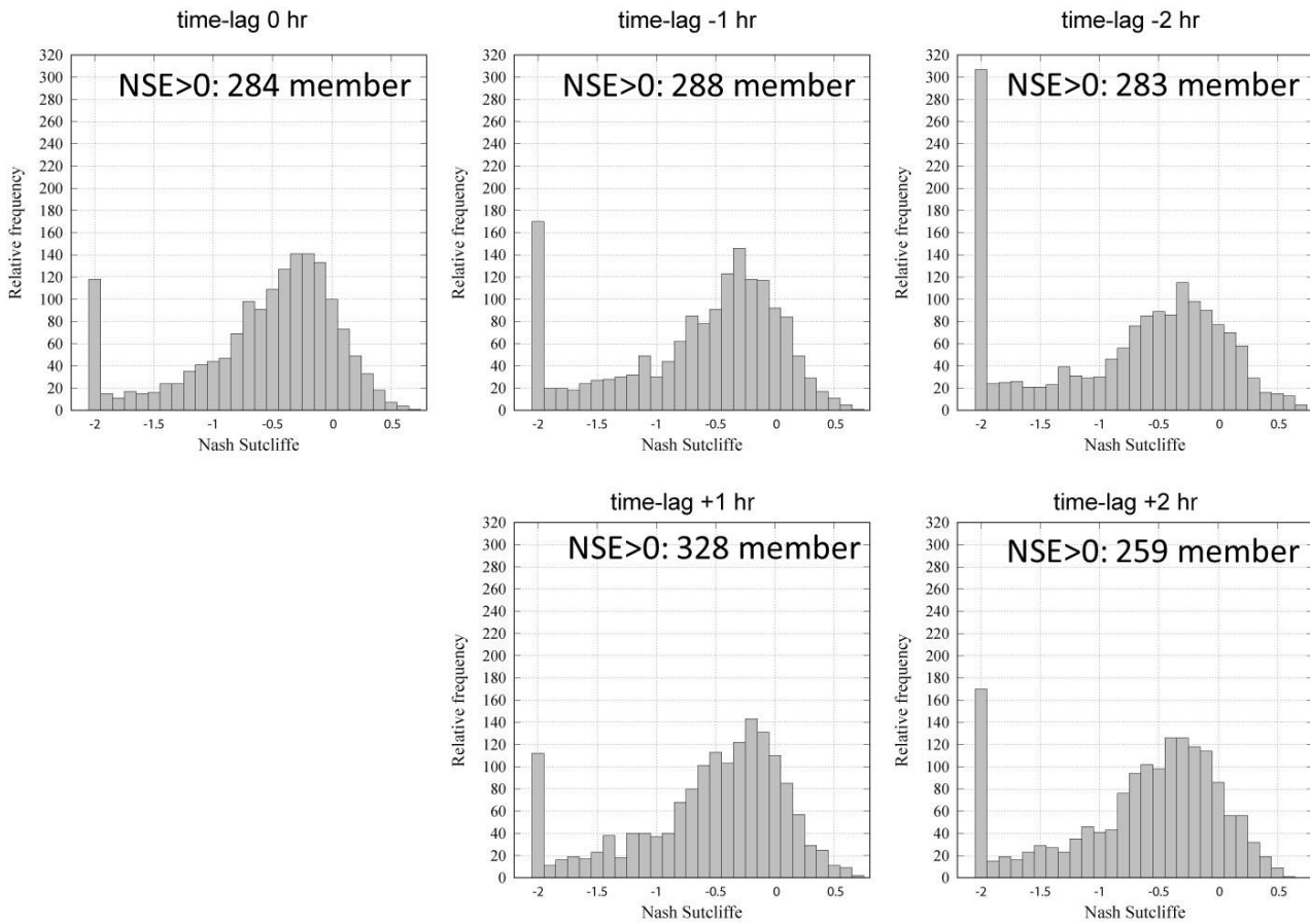
Figure S3 NSE considering the temporal displacement error
