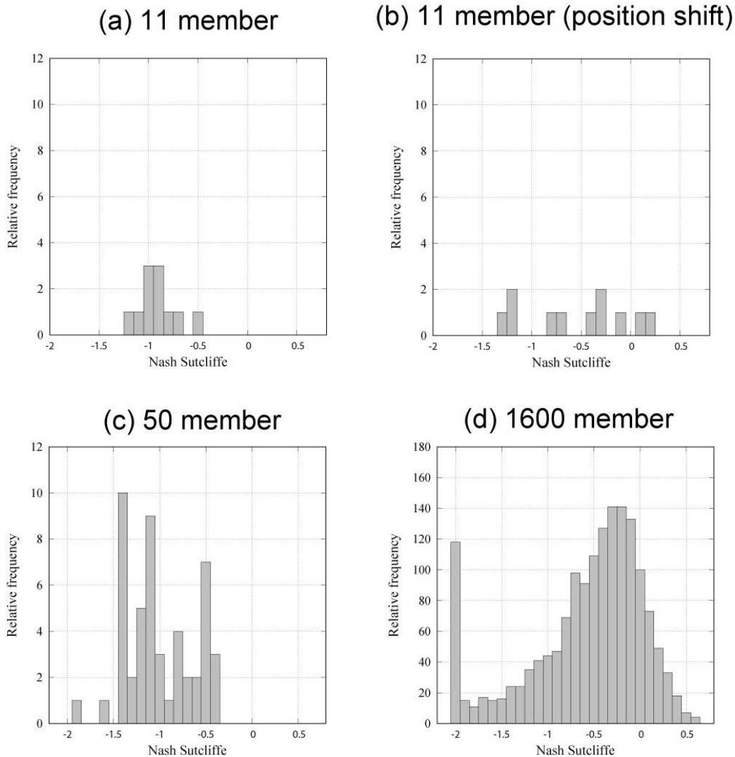
Figure S2: Histograms of NSE based on the simulated and observed discharges to Kasahori dam: (a) 11 discharge simulations in Part 1 (Kobayashi et al., 2016), (b) same 11 member but with a positional shift in Part 1 (Kobayashi et. al. 2016), (c) 50 discharge simulations with 4D-EnVAR-NHM and (d) 1600 discharge simulations with 4D-EnVAR-NHM.
