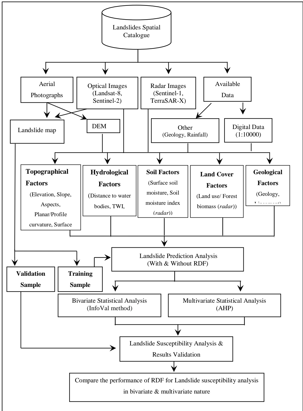
40 Figure 3 : Methodological Work flow of the Landslide susceptibility analysis using Bivariate and Multivariate approaches
