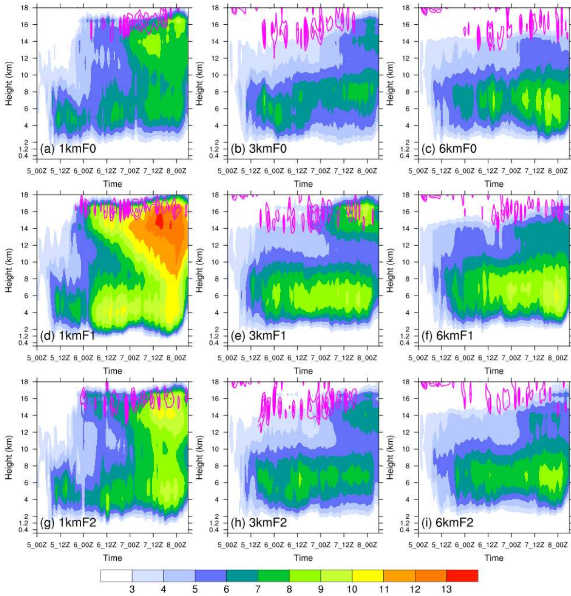
Figure 12. Time-height cross sections of upper level radial inflow (contours; \text{m s}^{-1} ) superposed on temperature anomaly (color shaded; \text{K} ) for experiments (a) 1kmF0, (b) 3kmF0, (c) 6kmF0, (d) 1kmF1, (e) 3kmF1, (f) 6kmF1, (g) 1kmF2, (h) 3kmF2, and (i) 6kmF2. The upper level radial inflows are contoured every 0.5 \text{ m s}^{-1} starting from -0.5 \text{ m s}^{-1} . The temperature anomaly is defined with respect to a composite of domain-averaged temperature profiles at the model initial time of the sensitivity experiments (0000UTC 5 November 2013); the composite of domain-averaged temperature profiles is derived as the mean of 8 domain-averaged temperature profiles obtained
