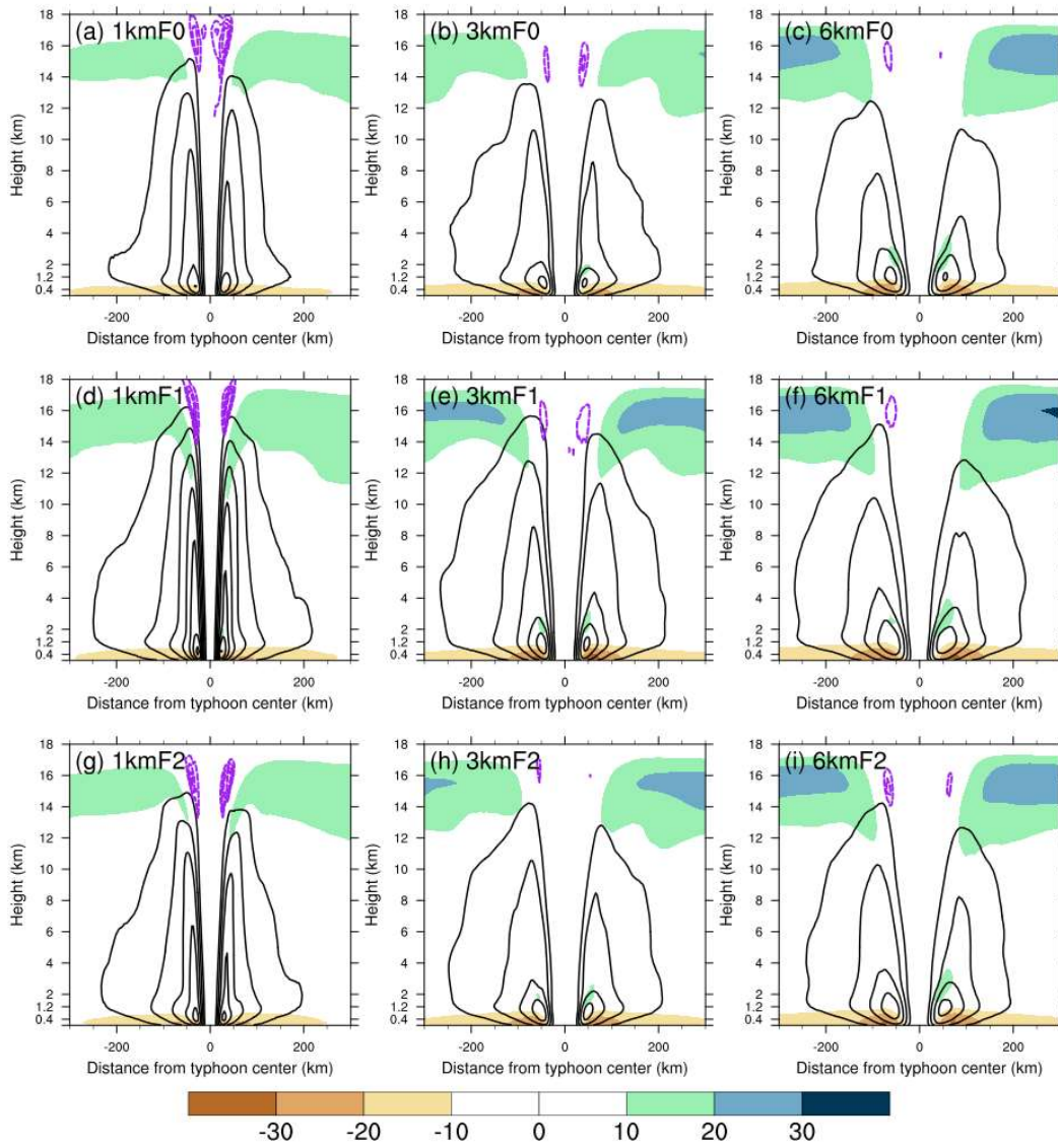
5 Figure 10. Radius–height cross sections of tangential wind (contours; m s^{-1} ) superposed on radial wind (color shaded; m s^{-1} ) for experiments (a) 1kmF0, (b) 3kmF0, (c) 6kmF0, (d) 1kmF1, (e) 3kmF1, (f) 6kmF1, (g) 1kmF2, (h) 3kmF2, and (i) 6kmF2. The tangential winds are contoured every 10 m s^{-1} starting from 30 m s^{-1} . Positive values of radial wind indicate inflow. The upper level radial inflows (purple dashed contours; m s^{-1} ) are also imposed and are contoured every 0.5 m s^{-1} starting from -0.5 m s^{-1} . All fields are time averaged between 1800UTC 7 November 2013 and 0000UTC 8 November 2013. Positive and negative distances represent the right (northern) and left (southern) semicircles as in Fig. 7.
