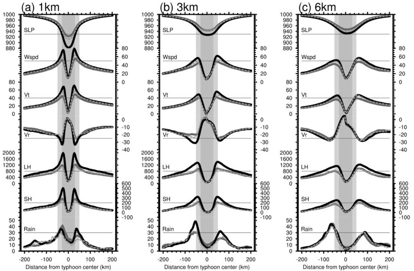
Figure 8. The radial variations of surface fields for experiments 1 km (left), 3 km (center), and 6 km (right). The surface fields shown are (from top to bottom) sea level pressure (SLP; hPa), wind speed and tangential and radial winds at 10 m (Wspd, Vt, and Vr; \text{m s}^{-1} ), surface latent and sensible heat fluxes (LH and SH; \text{W m}^{-2} ), and total rainfall (Rain; \text{mm hour}^{-1} ). Positive values of Vr indicate inflow. Dim-gray, black, and gray-dashed curves represent flux options F0, F1, and F2, respectively. Horizontal gray lines are selected reference lines for each field. All fields are time averaged between 1800UTC 7 November 2013 and 0000UTC 8 November 2013. Positive and negative distances represent the right (northern) and left (southern) semicircles as in Fig. 7. Vertical light-gray and gray shaded bars denote the radial sectors bounded by radii of 50 km and 30 km, respectively.
