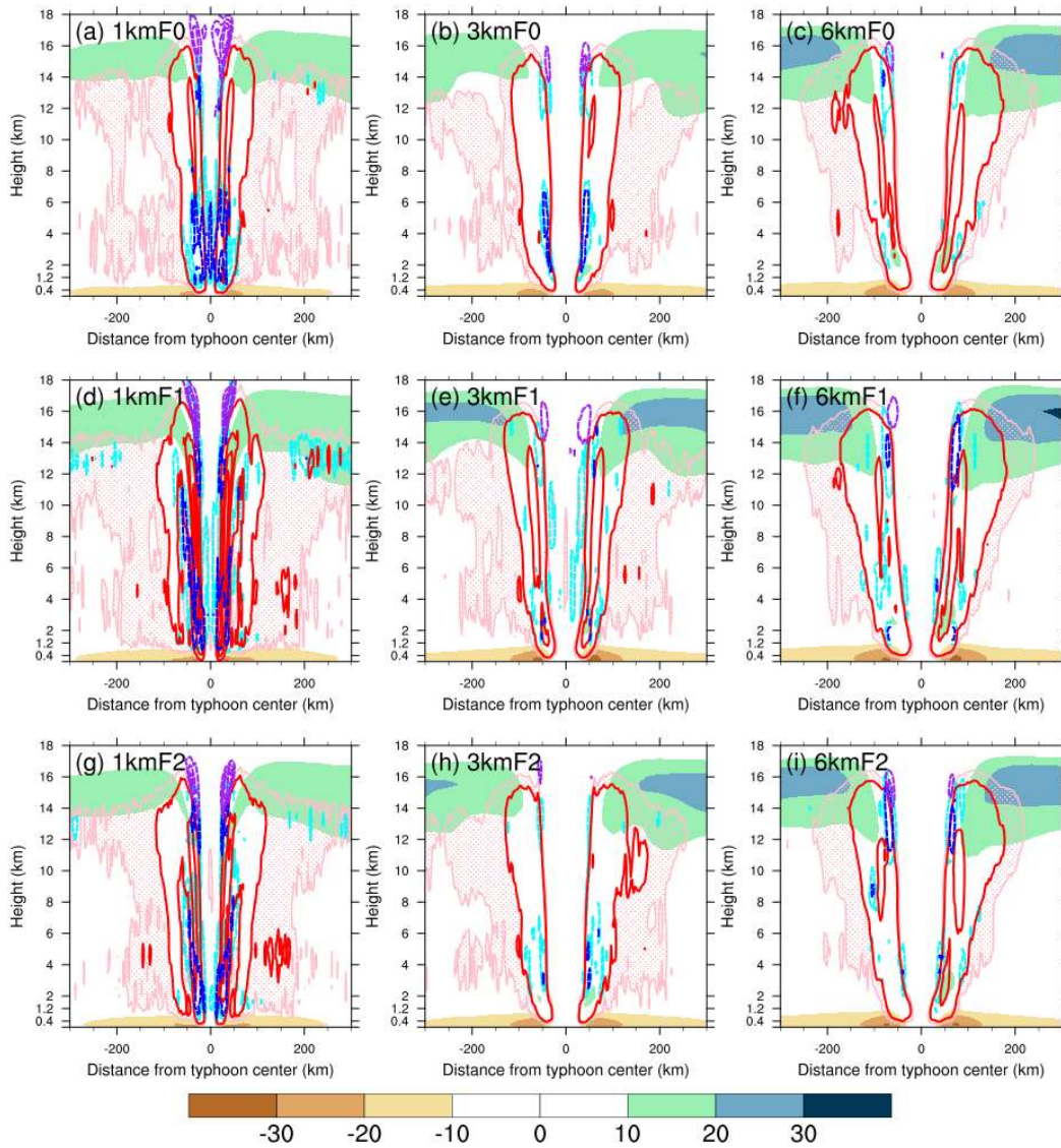
Figure 11. The same as Fig. 10 but for vertical velocity (contours; \text{m s}^{-1} ) and radial wind (color shaded; \text{m s}^{-1} ).
