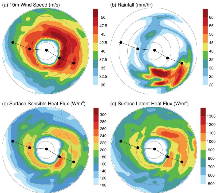
5 Figure 5. Horizontal distributions for (a) wind speed ( m s^{-1} ) at 10-m height, (b) total rainfall ( mm hour^{-1} ), (c) surface sensible heat flux ( W m^{-2} ), and (d) surface latent heat flux ( W m^{-2} ) at forecast hour 71 h (valid at 2200UTC 7 November) for the experiment F0 with 3-km resolution. All fields are taken from the transformed subset on cylindrical grids; see text for detail. At 71 h, the simulated typhoon centered at the nearest location upon the best-track location at 1800UTC 7 November 2013. Range rings are shown at radii of 20, 40, 60, 80, and 100 km. Black dot at the plane center denotes the simulated typhoon center at 71 h, whereas the two dots to the upper left and lower right of this central dots are the corresponding locations of typhoon center in the next and previous 2 10 hours. Solid lines connecting these dots denote the simulated typhoon track within the 5 hours.
