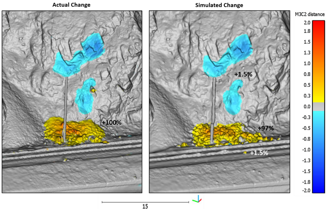
Figure 16: A comparison of the actual and simulated change detection results from the 8 m 3 planar sliding event from White Canyon West, Site E. The simulation produced a good comparison with the actual change detection results, yielding a similar spatial distribution and magnitude of change. The percentage of initial source volume retained at various locations on the actual and simulated slope is shown. The majority of material in both cases is retained in the track-side ditch. In the simulated case a small amount of the simulated volume comes to rest on the slope (1.5%) and runs out into the track area (1.5%).
