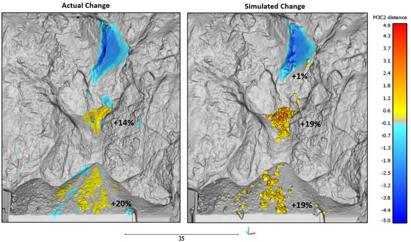
Figure 12: A comparison of the actual and simulated change detection results from the 170 m 3 wedge sliding event at Goldpan, Site A. The simulation produced a good comparison with the actual change results, yielding a similar spatial distribution, and magnitude of change. In both cases accumulation takes place on the mid-slope bench and on top of the rock shed, with the majority of material running out over the shed and off the slope. The percentage of initial source volume retained at various locations on the actual and simulated slope is displayed and shows a strong agreement. Areas of additional loss in the actual change detection, on top of the rock shed and at the mid-slope bench, are not captured in the simulation results. The simulation technique uses a fixed, rigid slope surface, and is not able to capture smaller slope failures which may have occurred as a result of talus impacts during the initial 170 m 3 event.
