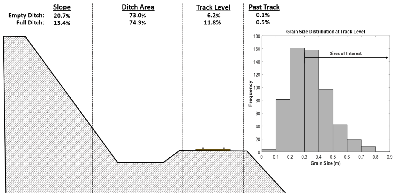
Figure 21: A schematic overview of the volume percentages stopping at different locations for the 15 simulation iterations using the empty and full ditch geometries. Simulation using the full ditch geometry resulted in nearly twice as much material reaching track level. The distribution of the grain sizes which reached track level in the full ditch scenario is also shown.
