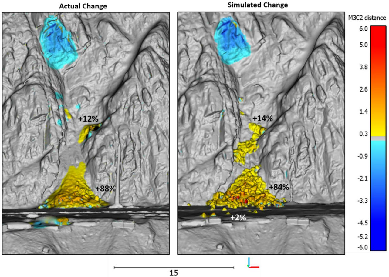
Figure 13: A comparison of the actual and simulated change detection results from the 24 m 3 wedge sliding event from White Canyon East, Site B. The simulation produced a good comparison with the actual change results, yielding a similar spatial distribution, and magnitude of change. The percentage of initial source volume retained at various locations on the actual and simulated slope is shown. In this case the majority of material in both the actual and simulated analysis ends up in the track-side ditch, with a smaller component of the volume stopped inside the gully. In the simulated change a small number of fragments do reach track level, representing approximately 2% of the simulated volume.
