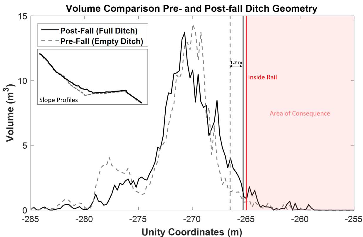
Figure 20: The distribution of simulated volume for the pre-fall and post-fall ditch geometries is shown. The vertical grey and black lines indicate the 95% volume-runout boundaries for the two cases. Simulation using the post-fall (full) ditch geometry results in the 95% volume-runout boundary shifting 1.2 m closer to the inside rail.
