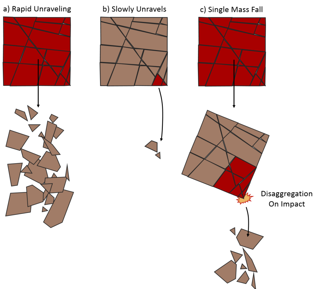
Figure 22: Comparing potential timing of rockmass fragmentation, which could have taken place for the events discussed. Red block indicate material which breaks away from the initial source volume at a given time.
