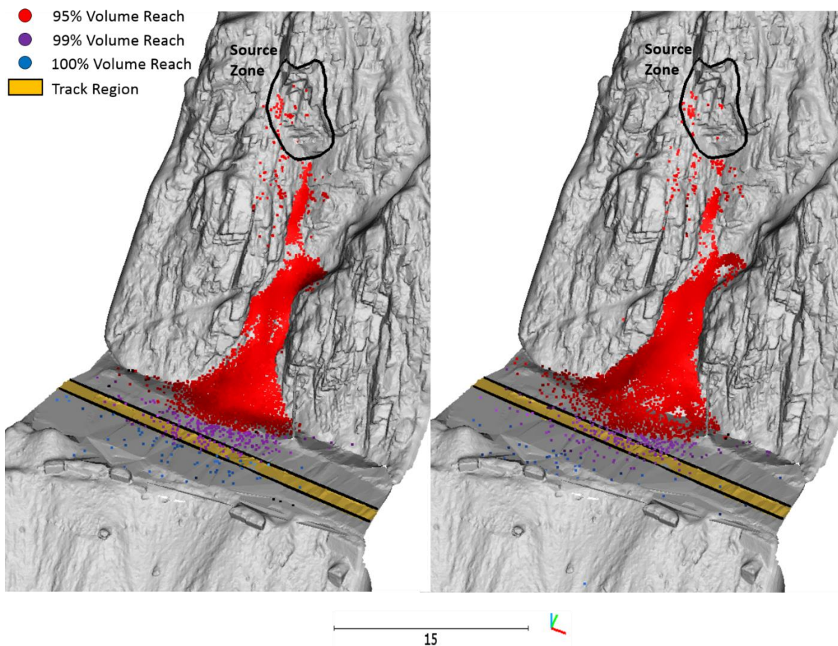
Figure 19: Comparison of the 15 simulation iterations of the 24 m 3 wedge sliding event at Site B using the pre-fall (empty) and post-fall (full) ditch geometries. In the full ditch scenario the 95% and 99% runout boundaries have shifted further forward into the track area, indicating a decreased effectiveness in the ditch at stopping material from reaching the track.
