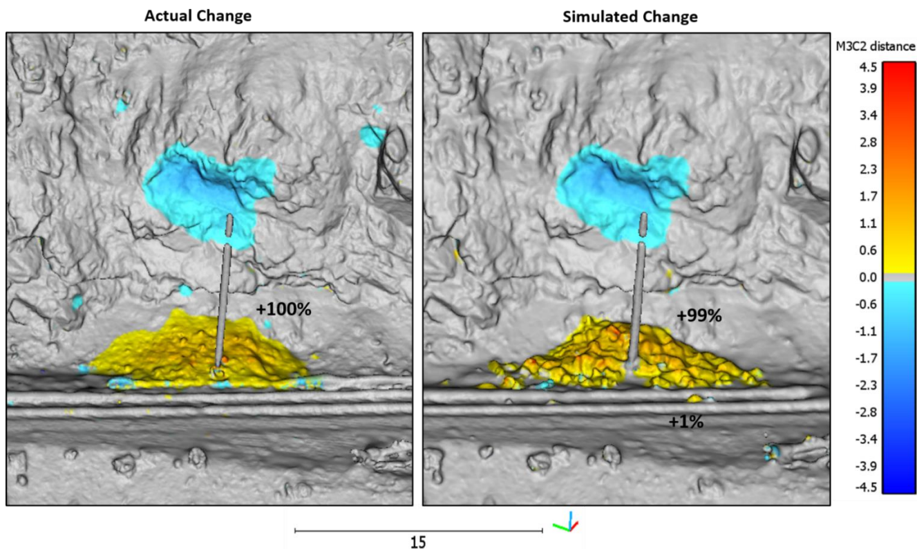
Figure 15: A comparison of the actual and simulated change detection results from the 15 m 3 planar sliding event from White Canyon West, Site D. The simulation produced a good comparison with the actual change detection results, yielding a similar spatial distribution, and magnitude of change. The percentage of initial source volume retained at various locations on the actual and simulated slope is shown. The majority of material in both cases is retained in the track-side ditch. In the simulated case, 1% of the volume reaches the track area.
