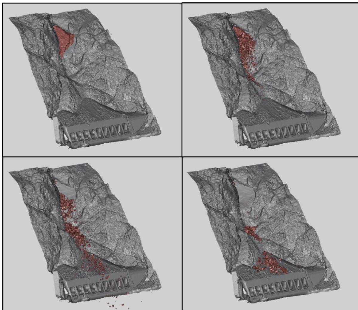
Figure 11: Screenshots of a fragmental rockfall simulation (1000 fragments) for the 170 m 3 rockfall event at Goldpan.
