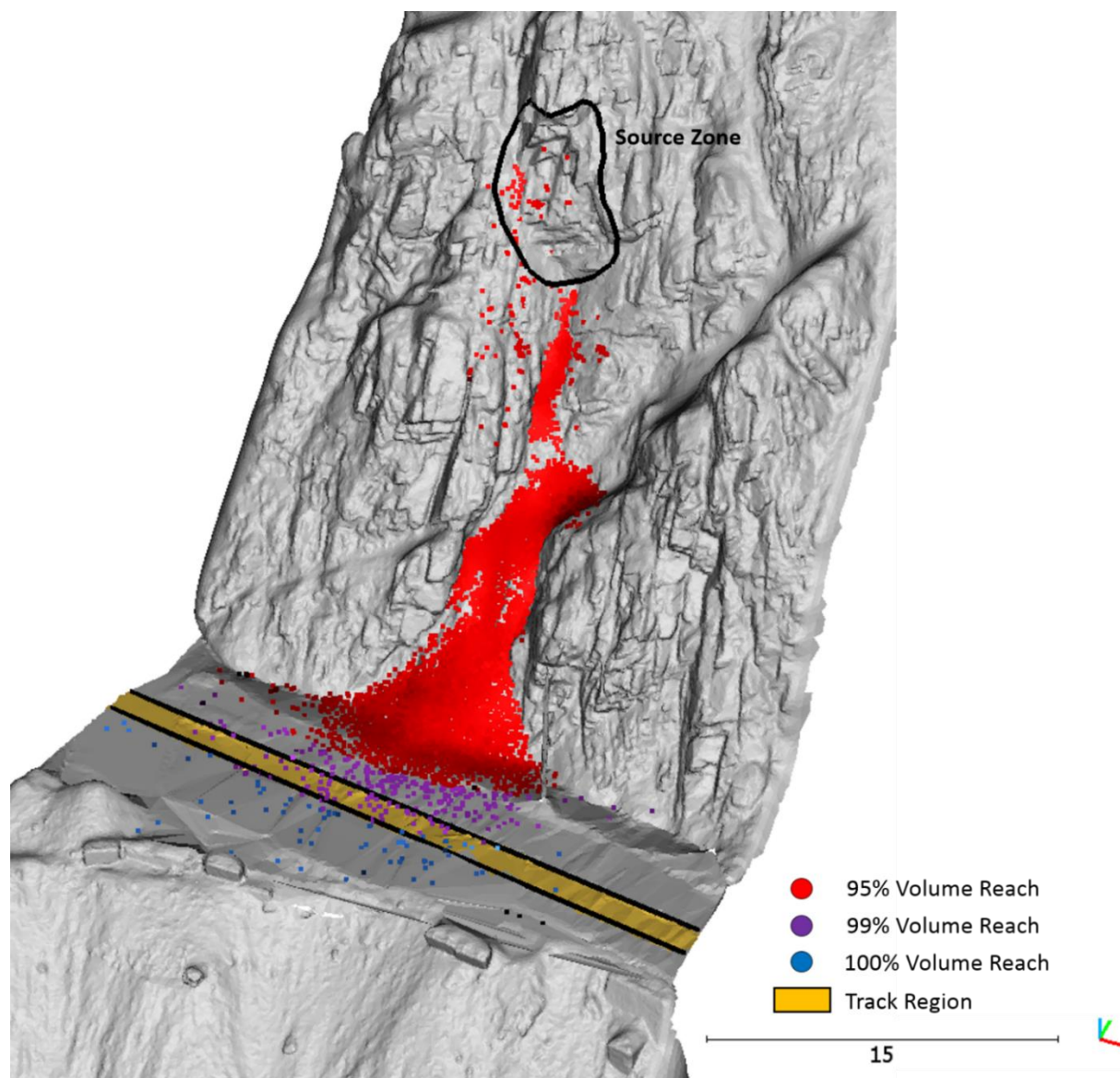
Figure 17: Results of the 15 simulations run for the 24 m 3 wedge sliding event at White Canyon East, Site B. Each point represents the end point of a simulated fragment in one of the 15 simulations. The envelope of red points indicates the runout of 95% of the simulated volume, with the purple and blue portions representing envelopes containing the additional 4% and 1% of the material, respectively.
