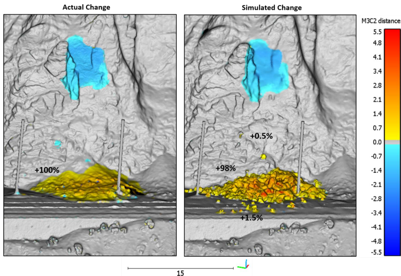
Figure 14: A comparison of the actual and simulated change detection results from the 32 m 3 flexural toppling event from White Canyon East, Site C. The simulation produced a good comparison with the actual change detection results, yielding a similar spatial distribution, and magnitude of change. The percentage of initial source volume retained at various locations on the actual and simulated slope is shown. The majority of material in both cases is retained in the track-side ditch. In the simulated case a small amount of the simulated volume comes to rest on the slope (0.5%) and runs out into the track area (1.5%).
