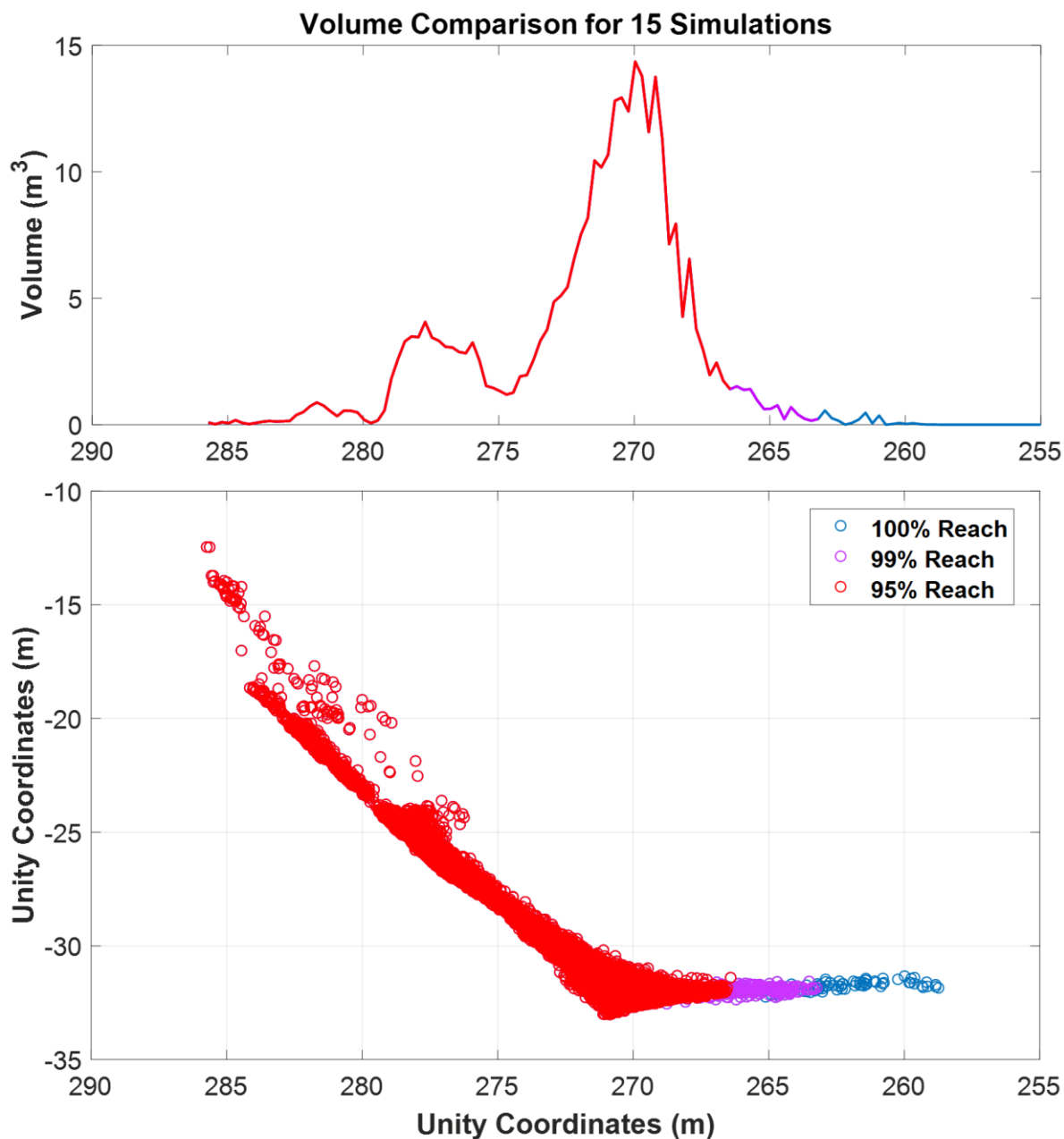
Figure 18: A section view of the 15 simulation iterations run for the 24 m 3 wedge sliding event at White Canyon East, Site B. The top plot shows the accumulation of simulated fragments across the section. The notable peak visible at 270 m is in alignment with the location of the track-side catchment ditch, as shown in the lower plot.
