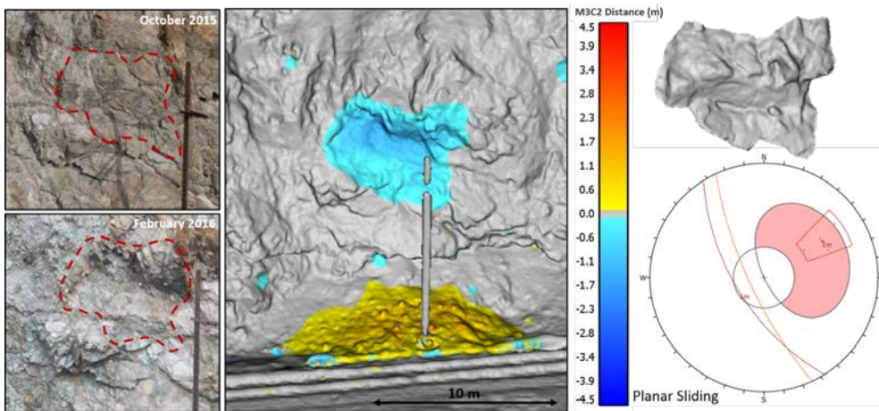
Figure 6: Site D. Schematic overview of the 15 m 3 planar sliding rockfall event detected at the White Canyon West site between October 2015 and February 2016. The event involved an irregularly shaped slab of weathered and heavily jointed rockmass which failed approximately 9.5 m above track level. Site photos (left) of the source zone pre- and post-failure are shown. Change detection results of the event are shown (center) with cool colours indicating material loss and warm colours indicating material accumulation. Change detection results indicate that the bulk of the material from the event was retained by the track-side ditch. The rockfall hull of the event, extracted from the pre- and post-failure meshes is shown (upper right), as well as a stereo-net representation of the planar sliding failure mode.
