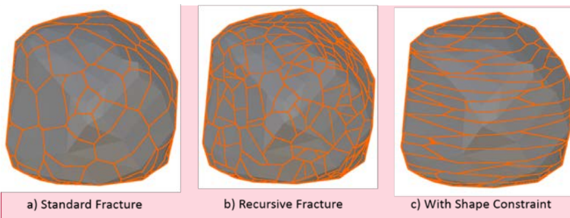
20 Figure 11: Showing the results of different Voronoi fracturing methods. Recursive fracturing in b) results in the additional fracturing of the initial convex polyhedra in a). Shape constraints in c) result in the elongation of the convex polyhedra, creating a more sheet-like fracture network.
