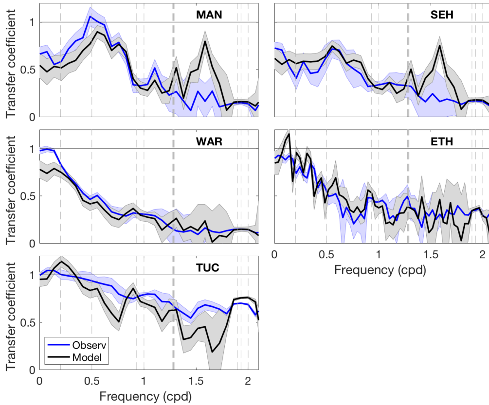
520 Figure 5. Comparison between observed (blue) and numerical model (black) transfers for the period when both are available (March-December 2012) at five bay stations. Uncertainty envelopes for the transfer coefficient (Bendat and Piersol, 1986) are provided for observed (light blue) and model (gray) estimates.
