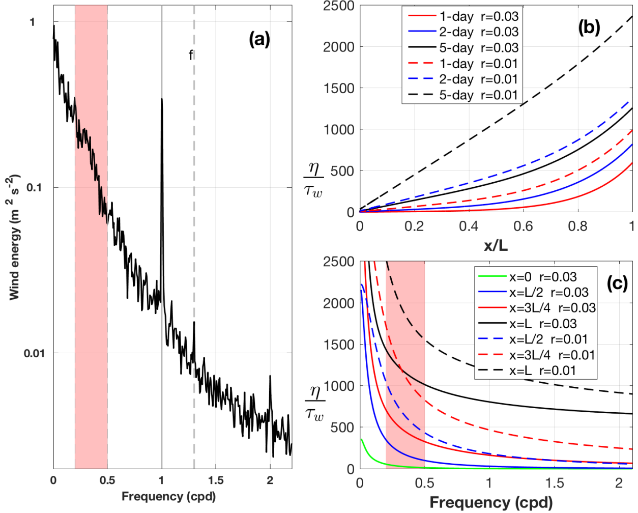
530 Figure 7: (a) Wind speed spectra for the along-bay wind component for NDBC 44065 buoy (2008-2018). (b) Kinematic wind stress contribution to local water level in the bay expressed as \frac{\eta}{\tau_w} ( \text{m}^{-1}\text{s}^2 ) following the Wong and Moses-Hall (1998) formulation as a function of distance from the southern edge of the bay. (c) Kinematic wind stress contribution to water level as a function of frequency. The vertical shaded area indicates the frequencies corresponding to the storm band (2-5 days).
