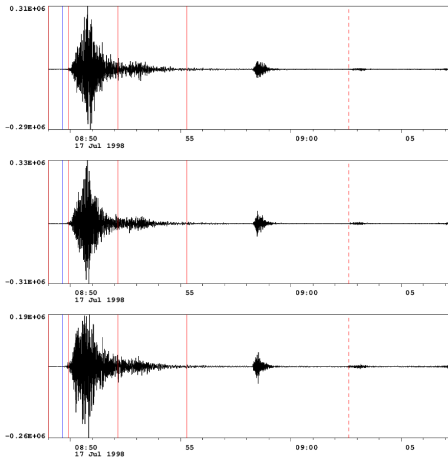
Fig. 1. High-pass filtered records at JAY
