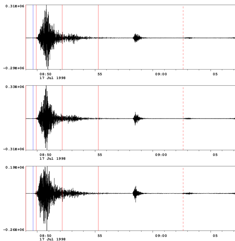
Fig. 1. High-pass filtered records at JAY
