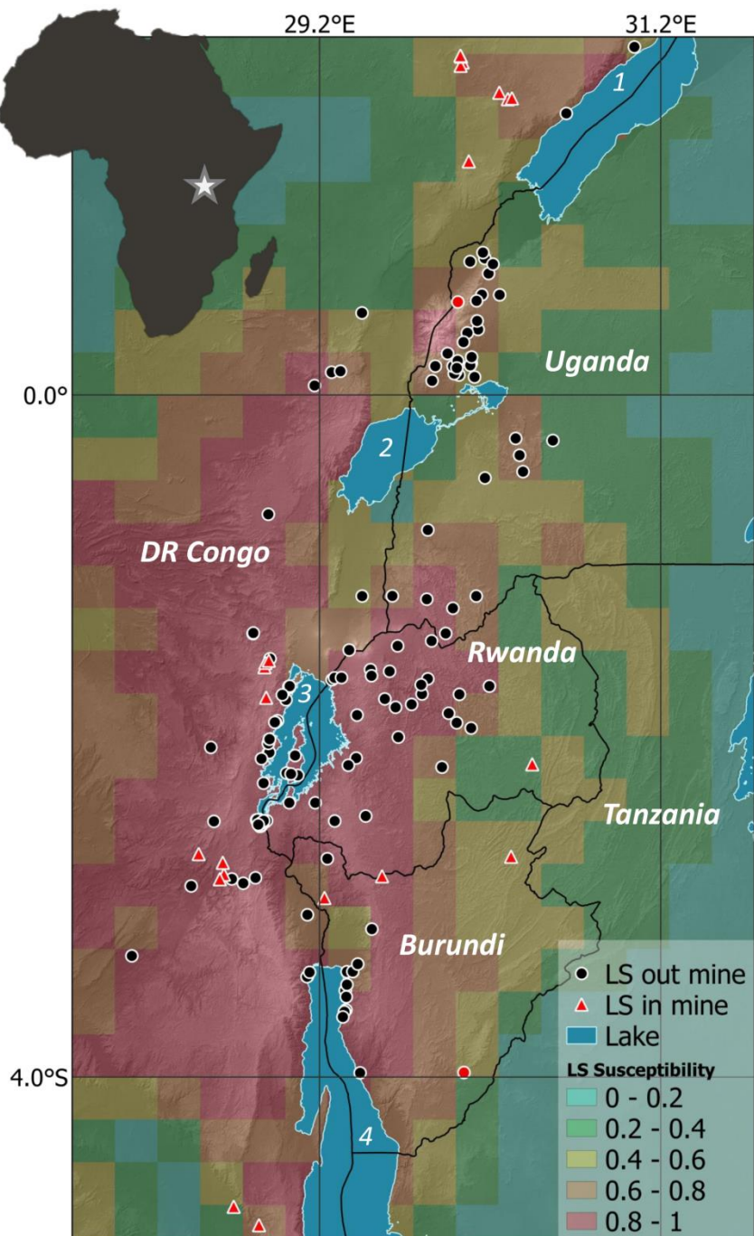
Figure 1. Landslide susceptibility at 0.25^\circ resolution, derived from the map of Broeckx et al. (2018), and distribution of landslides in the western branch of the East African Rift, comprising 29 landslides in mining areas (triangles), and 145 landslides outside mining areas (dots) of which the red dots are landslides associated with antecedent rainfall less than 5 mm. Only the black dots (143 landslides) are used for calibrating the rainfall thresholds. Numbers in the lakes: 1 = Lake Albert, 2 = Lake Edward, 3 = Lake Kivu, 4 = Lake Tanganyika. Background hillshade SRTM (90m).
