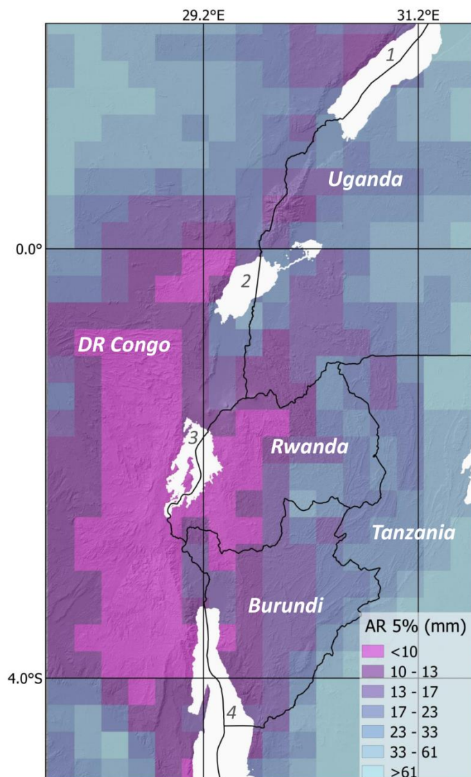
Figure 5. Antecedent rainfall (AR) threshold map ( 0.25^\circ resolution) at 5% exceedance probability (see Eq. 5). Depending on the local landslide susceptibility (from Broeckx et al. 2018, Fig. 1) threshold values range from AR = 9.5 mm in the highest-susceptibility areas ( S = 0.97 ) to AR = 23.1 mm in the least susceptible pixels ( S = 0.38 ) having recorded landslides during the 2001-2018 period. Numbers in the lakes: 1 = Lake Albert, 2 = Lake Edward, 3 = Lake Kivu, 4 = Lake Tanganyika. Background hillshade SRTM (90m).
