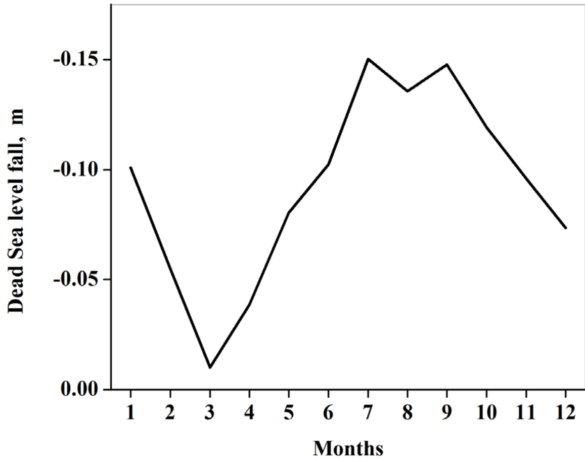
Figure 9: 17-year (2000 – 2016) mean seasonal variations of the Dead Sea water-level drop estimated separately for each month.
