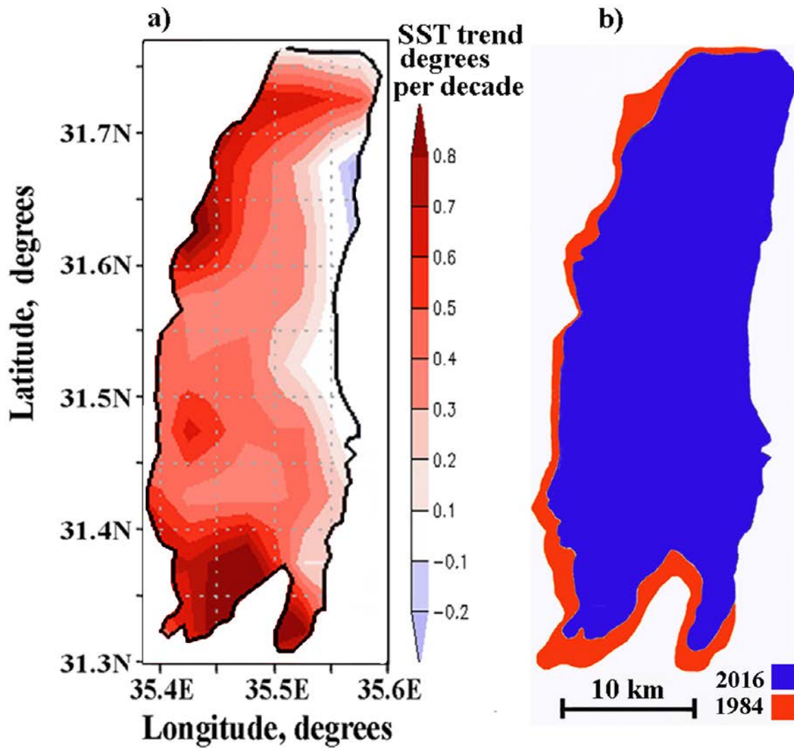
5 Figure 13: a - Spatial distribution of 17-year trends of daytime Dead Sea SST ( ^{\circ}\text{C decade}^{-1} ) averaged over the JAS summer months: July, August, and September. b - The Dead Sea water area in the two years: 1984 and 2016, based on data from the Google Earth Engine (Gorelick et al., 2017).
