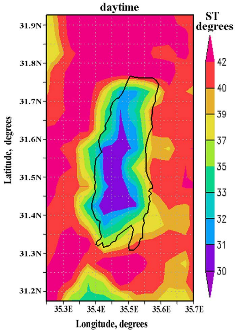
Figure 11: Spatial distribution of 17-year mean daytime surface temperature (ST, °C) over the Dead Sea and surrounding land areas, averaged over the JAS summer months: July, August, and September.
