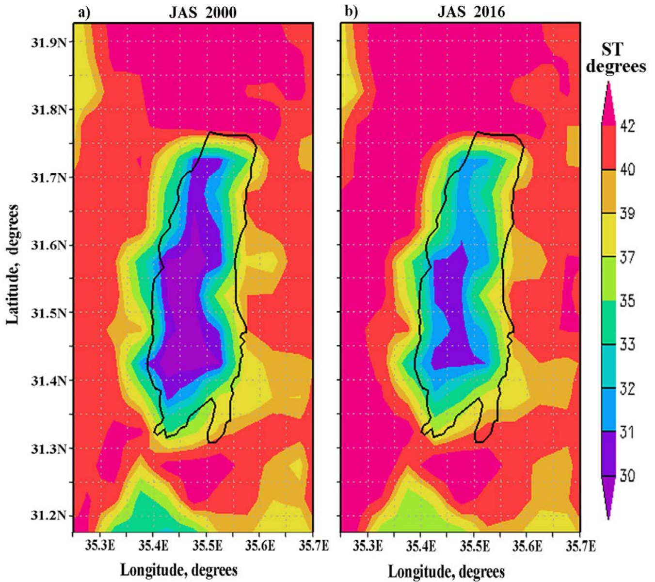
Figure 12: Comparison of the spatial distribution of daytime surface temperature (ST, °C) over the Dead Sea and surrounding land areas (averaged over the JAS summer months) between the years of 2000 and 2016.
