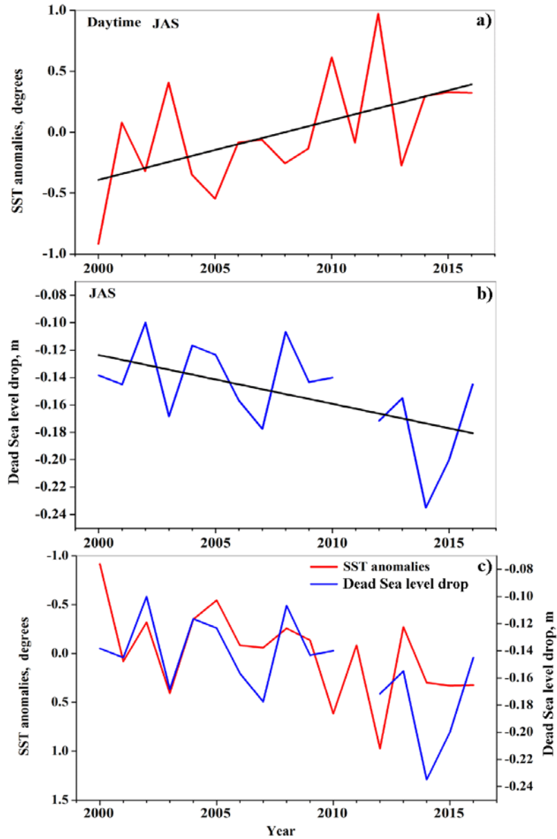
5 Figure 10: Year-to-year variations in (a) daytime SST anomalies and (b) Dead Sea water-level drop, averaged over the three summer months July, August, and September (JAS) characterized by the largest Dead Sea water-level drop. c is a comparison between the temporal variations in daytime SST anomalies and Dead Sea water-level drop averaged over the same three summer months. For illustrative purposes, the decreasing scale of SST anomalies is used in (c) instead of the increasing scale used in (a). One can see that these variations are correlated representing an inverse relationship.
