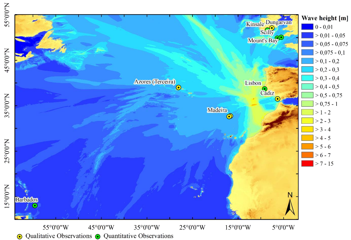
Figure 4. Maximum wave height distribution (color scale in m) in the Atlantic basin produced by the source of hypothesis A-MS.
