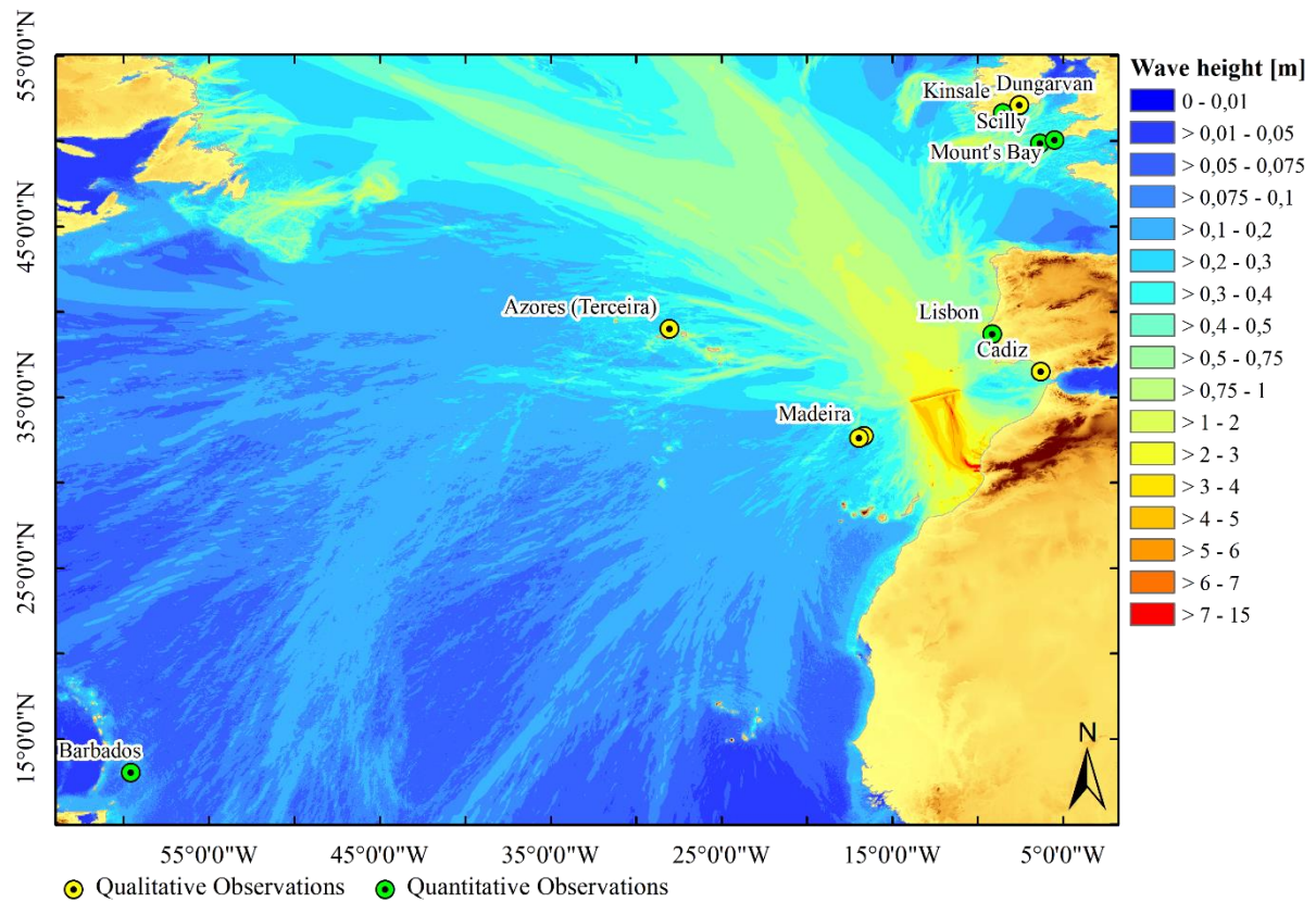
Figure 6. Maximum wave height distribution (color scale in m) in the Atlantic basin produced by the source of hypothesis B.
