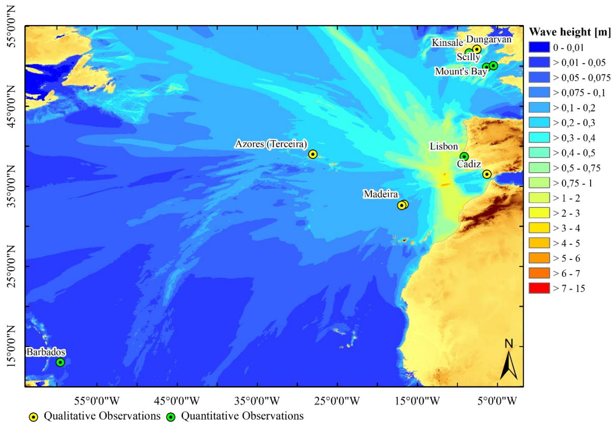
Figure 4. Maximum wave height distribution (color scale in m) in the Atlantic basin produced by the source of hypothesis A-MS.
