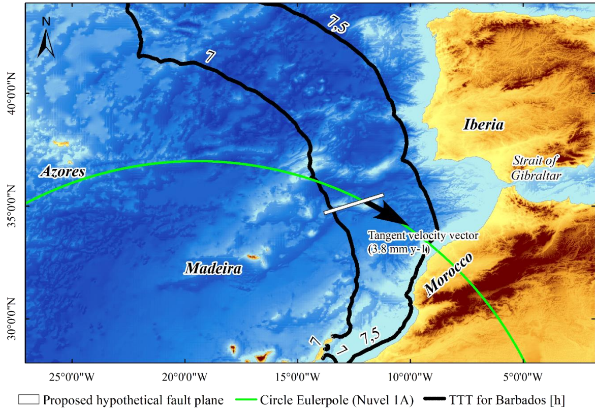
Figure 3. Circle around the Euler pole at the proposed hypothetical fault location. The model Nuvel 1A (DeMets et al., 1994, 1999) computes a 3.8 mm y -1 convergence. We plot the tangent velocity vector at the proposed fault. The black lines depict the backward ray tracing contours in hours, for TTT of 7-7.5 hours to Barbados.
