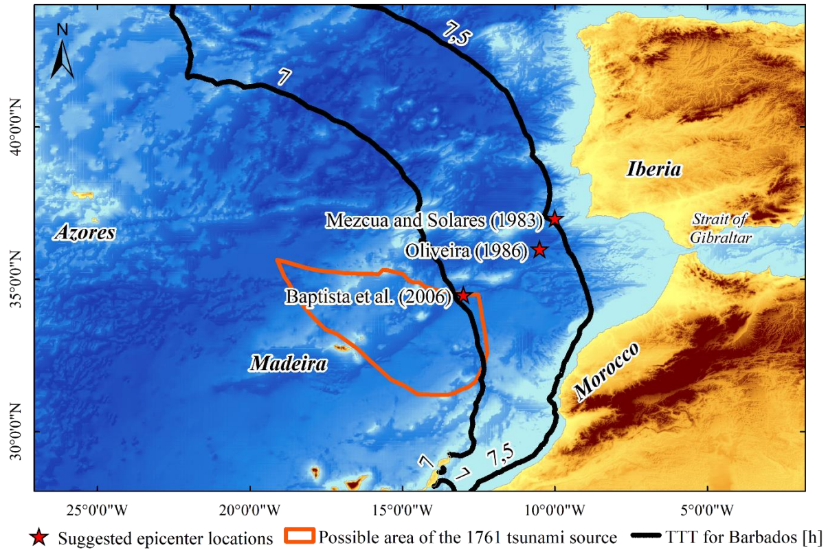
Figure 2. Source locations and backward ray tracing contours (black lines) for TTT of 7 – 7.5 hours to Barbados. The orange limited area defines the results obtained using macroseismic analysis combined with backward ray tracing but discarding the TTT for Barbados by Baptista et al. (2006).
