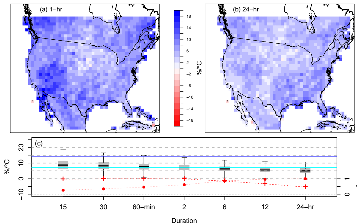
Figure 10. Temperature scaling of 10-yr return levels of (a) 1-hr and (b) 24-hr extreme rainfall; values shown are aggregated 100-km × 100-km grid box means. (c) Boxplots summarizing the distribution of temperature scaling values for 10-yr return levels of 15-min to 24-hr duration extreme rainfall. The horizontal line in the middle of each box indicates the median, boxes extend from the lower quartile to the upper quartile, and the whiskers to 1.5 times the IQR. The horizontal cyan (blue) line indicates temperature scaling of 7%/°C (14%/°C.) The red dashed (dotted) lines and the secondary vertical axis indicate the spatial correlation between maps of temperature scaling for each duration and the 1-hr (24-hr) maps.
