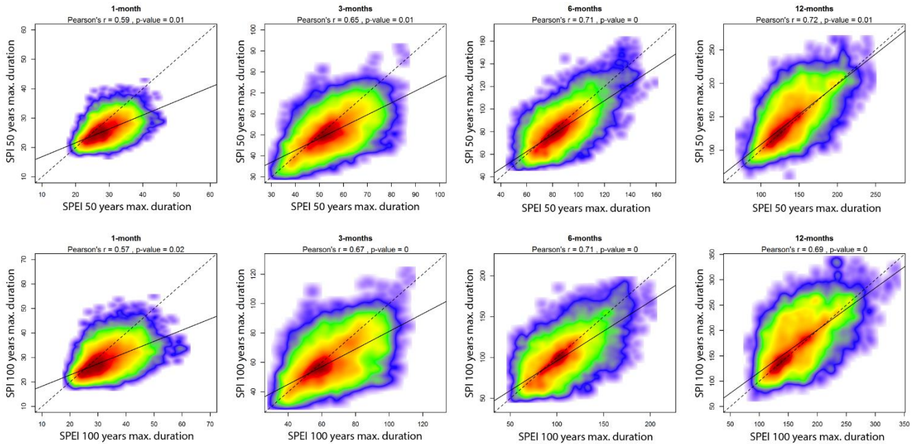
Figure 11: Scatterplots showing the relationship between the maximum drought duration (in weeks) expected in a period of 50 and 100 years considering 1-, 3-, 6- and 12- SPEI and the SPI. The colours represent the density of points, with red denoting the highest density. Given the large sample used, the significance of the Pearson's r coefficients was estimated by means of a Montecarlo approach using 10^3 random samples, with each sample containing 30 cases.
