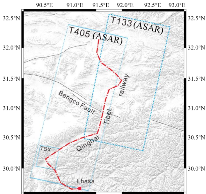
Figure 2. Study area and the distribution of the SAR imagery. The base map is derived from a digital elevation model (DEM). The blue dotted line shows the extents of the ASAR and TerraSAR-X images, the T405 and T133 represents the coverage of ASAR data, and the TSX represents the coverage of TerraSAR-X data. The red dotted line shows the railway. The black line shows the main fault in this area.
