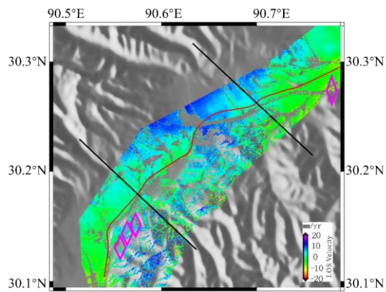
5 Figure 9. Deformation and hazards. The magenta rhombi show the geological hazard points.
