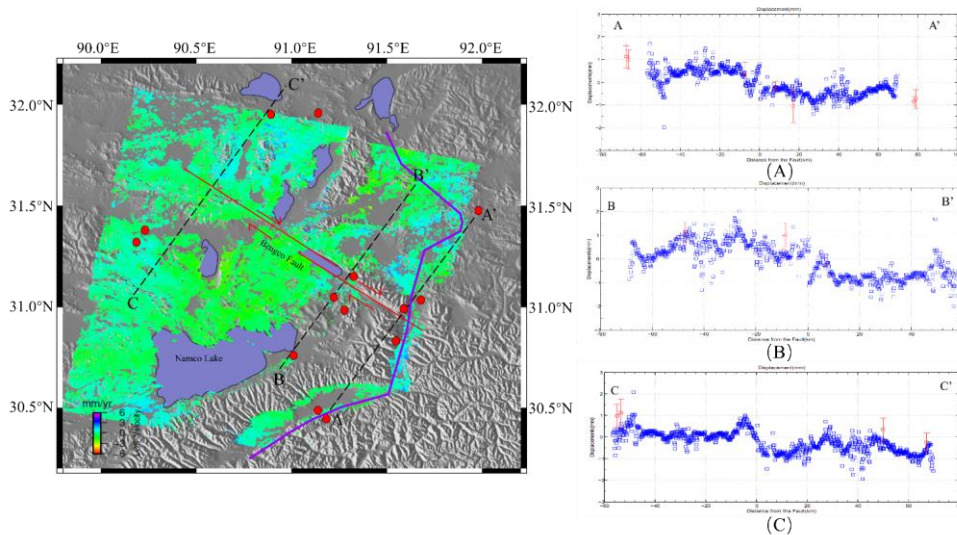
Figure 11. Bengo fault slip rate. The red line shows the Bengo fault. The purple line shows the railway. The red circle shows the GPS location. The black dotted line shows the profiles of the Bengo fault. The purple line shows the highway. The left figure shows the Bengo fault slip rate. The right figure shows the detailed information on profiles.
