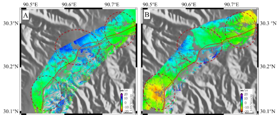
Figure 6. The deformation maps of the overlap area of the TerraSAR-X and ASAR data. (A) The ASAR T405 data range from 2008 to 2010. (B) TerraSAR-X data range from 2011 to 2012.
