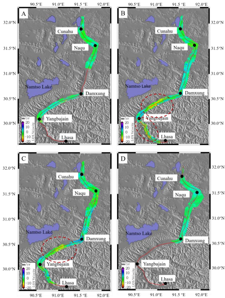
Figure 5. The InSAR results. Fig A represents the ASAR T405 results for the Lhasa-Naqu section of the Qinghai-Tibet Railway between 2003 and 2005. Fig B represents the ASAR T405 results for the Lhasa-Naqu section of the Qinghai-Tibet Railway in 2007, and the elliptical red dotted line represents the region of large deformation. Fig C represents the data are ASAR T405 data from 2008 to 2010. Fig D represents the data are ASAR T133 data from 2008 to 2010. The red line represents the railway. The black circle represents the main stations along the railway.
