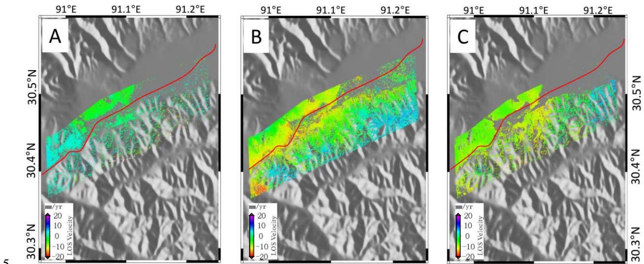
Figure 9. The deformation maps of the railway sequence changes from 2003 to 2010 in the Damxung section.
