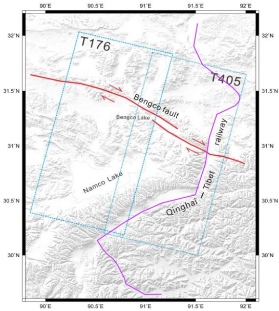
Figure 10. Bengo fault and the distribution of the SAR imagery. The blue dotted line shows the extents of the ASAR images. The red line shows the Bengo fault. The purple line shows the railway.
