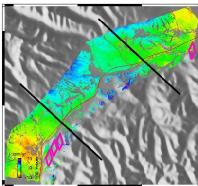
5 Figure 9. Deformation and hazards. The magenta rhombi show the geological hazard points.
