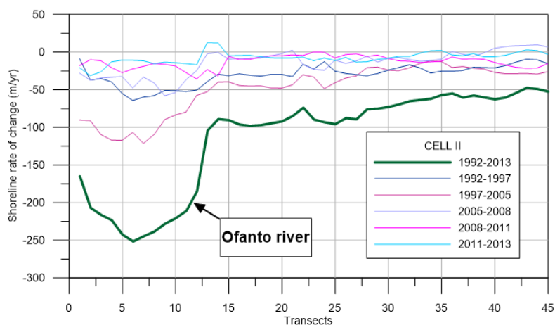
Figure 7: Shoreline evolution during 1992-1997, 1997-2005, 2005-2008, 1992-2013, 2008-2011, 2011-2013.
