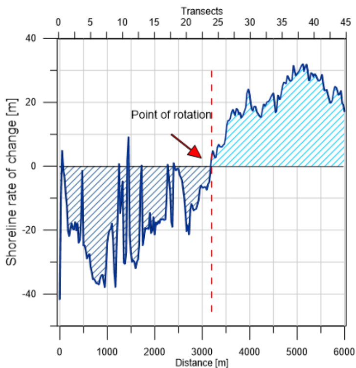
Figure 10: Shoreline change between 1992 and 2013 at Cell III. (Note: light area = accretion, dark area = erosion).
