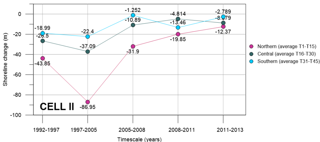
5 Figure 8: Average shoreline position in northern, central and southern sectors of Cell II.
