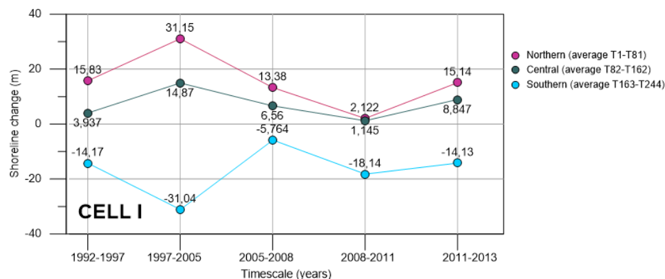
Figure 6: Average shoreline position in northern, central and southern sectors of Cell I.
