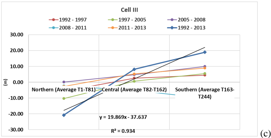
Figure 12: Average variation (m) at northern, central and southern shore in (a) Cell I, (b) Cell II and (c) Cell III for the years 1992-2013, 1992-1997, 1997-2005 and 2005-2008.
