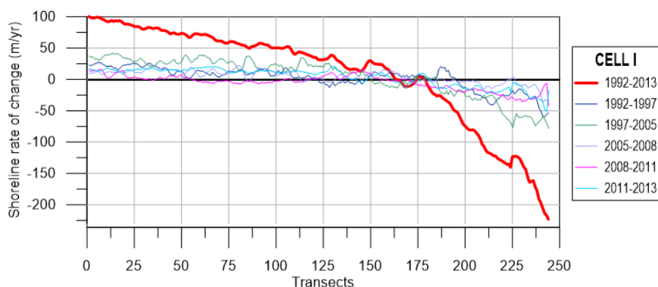
Figure 4: Shoreline evolution during 1992-1997, 1997-2005, 2005-2008, 2008-2011, 2011-2013.
