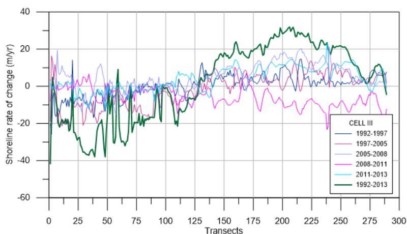
Figure 9: Shoreline evolution during 1992-1997, 1997-2005, 2005-2008, 1992-2013, 2008-2011, 2011-2013.
