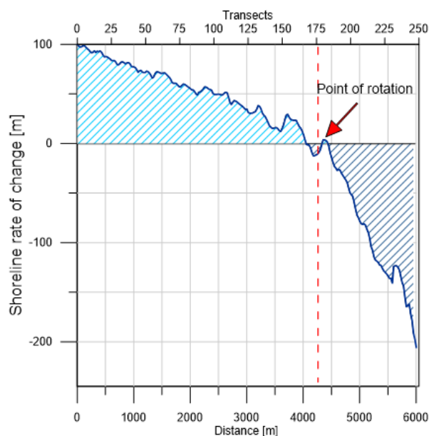
Figure 5: Shoreline changes between 1992 and 2013 at Cell I. (Note: light area = accretion, dark area = erosion).
