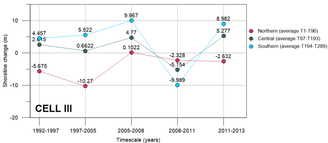
5 Figure 11: Average shoreline position in northern, central and southern sectors of Cell III.
