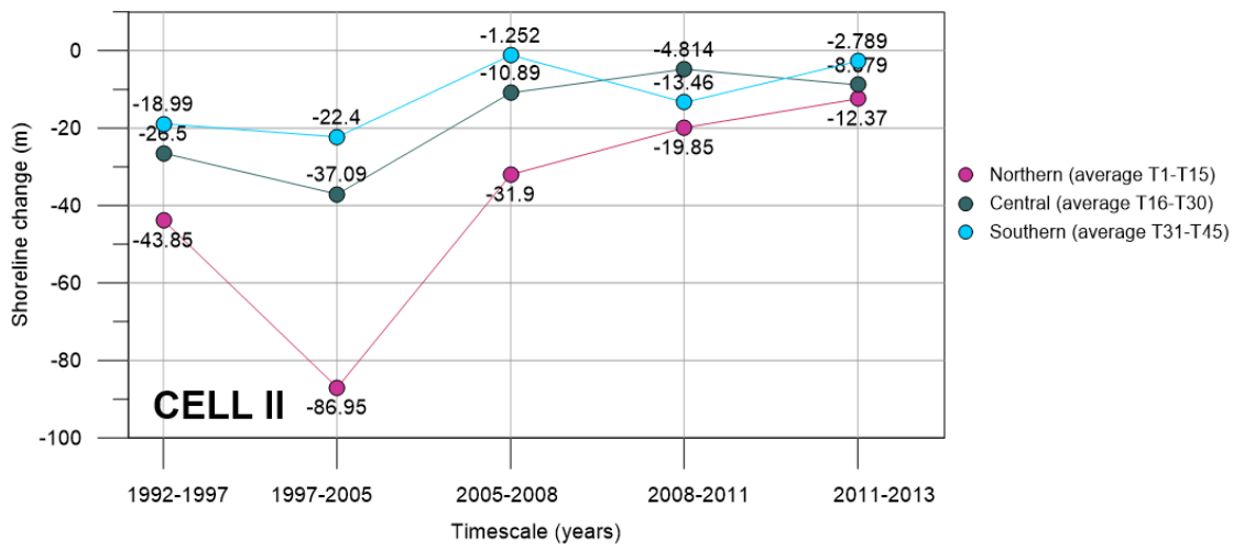
Figure 8: Average shoreline position in northern, central and southern sectors of Cell II.
