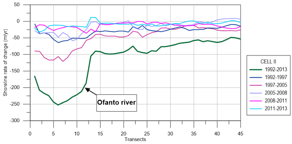
5 Figure 7: Shoreline evolution during 1992-1997, 1997-2005, 2005-2008, 1992-2013, 2008-2011, 2011-2013.
