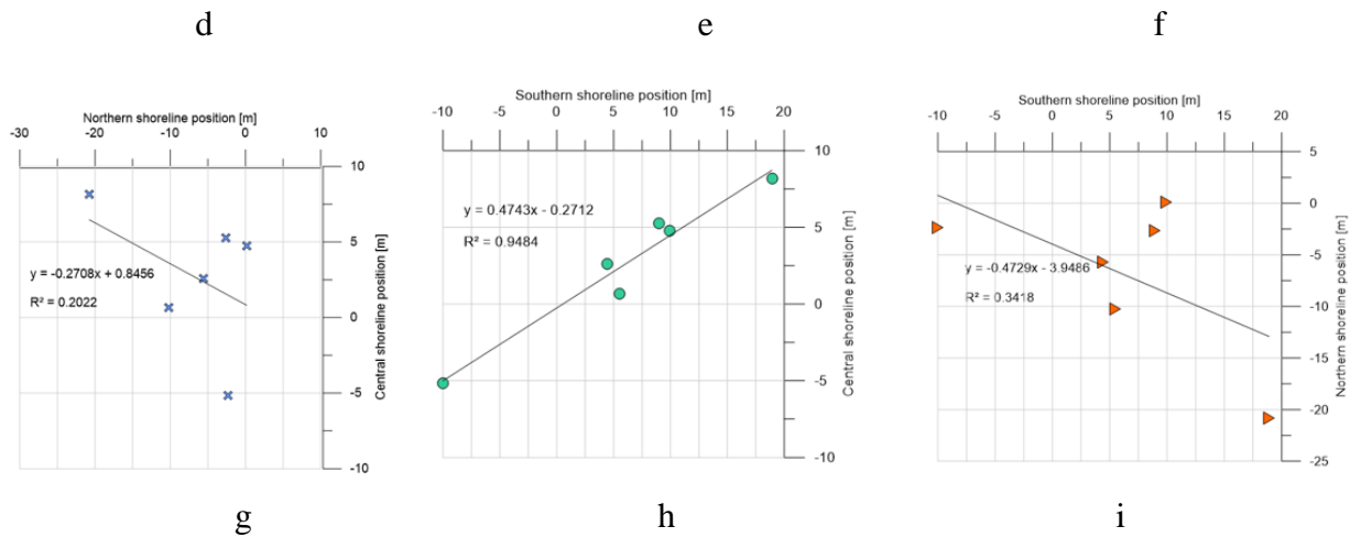
5 Figure 13: Spatial correlations of the averaged shoreline changes during the investigated period between: northern and central shoreline; southern and central shoreline; southern and northern region in Cell I (a), (b), (c), Cell II (d), (e), (f) and Cell III (g), (h), (i).
