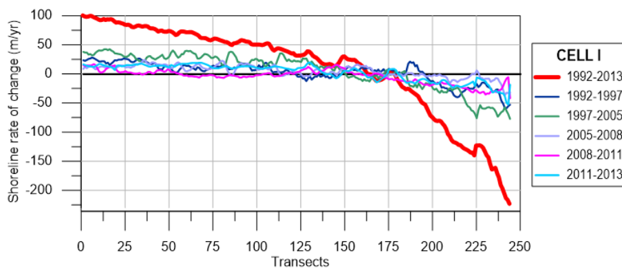
Figure 4: Shoreline evolution during 1992-1997, 1997-2005, 2005-2008, 2008-2011, 2011-2013.
