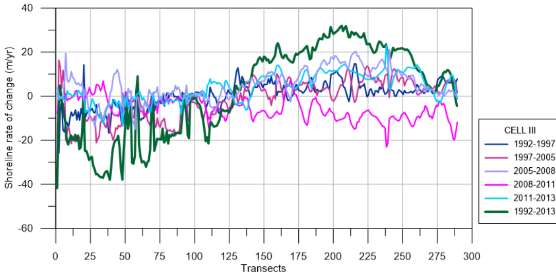
20 Figure 9: Shoreline evolution during 1992-1997, 1997-2005, 2005-2008, 1992-2013, 2008-2011, 2011-2013.
