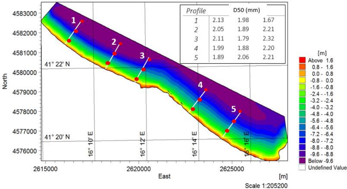
20 Figure 3: Bathymetry of the study area (Gauss-Boaga coordinates) and cross-shore model profiles. Mean diameters (D50) measured in three locations along each profile are reported (from the coast to open sea).
