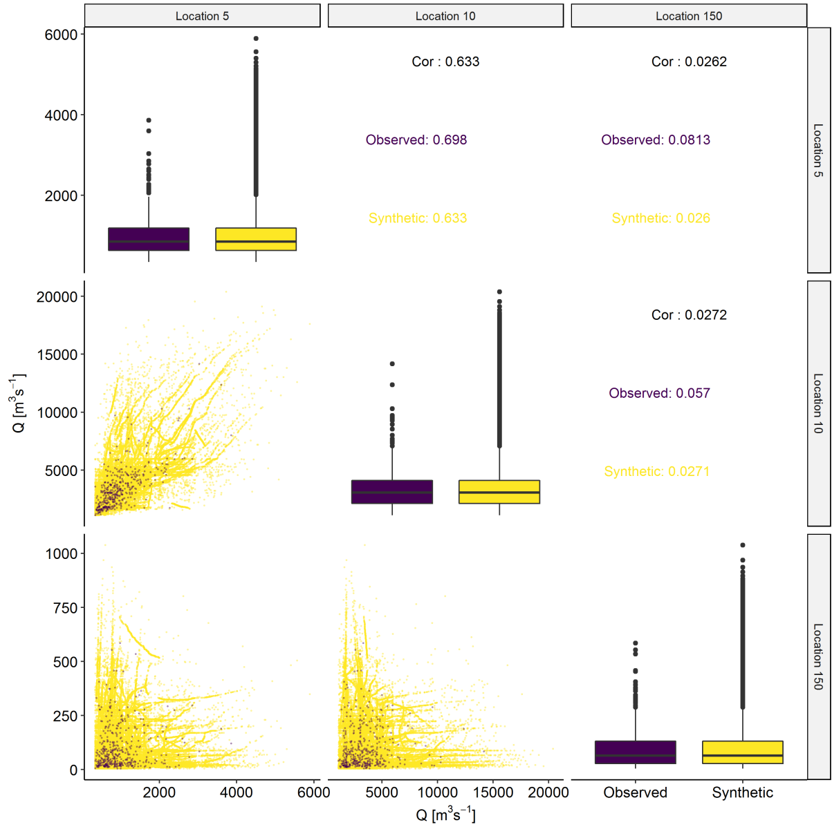
Figure 7. Observed (purple) versus synthetic (yellow) descriptors at three locations. In the diagonal, distributions of observed and synthetic descriptors per location are compared using box-plots. Below the diagonal, pair-wise scatter plots are displayed. Above the diagonal, pair-wise correlations are displayed.
