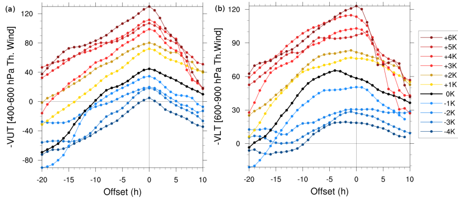
Figure 9. Composite time series of (a) -V_T^U and (b) -V_T^L from -20 h before to +10 h after MWCT for each SST change.
