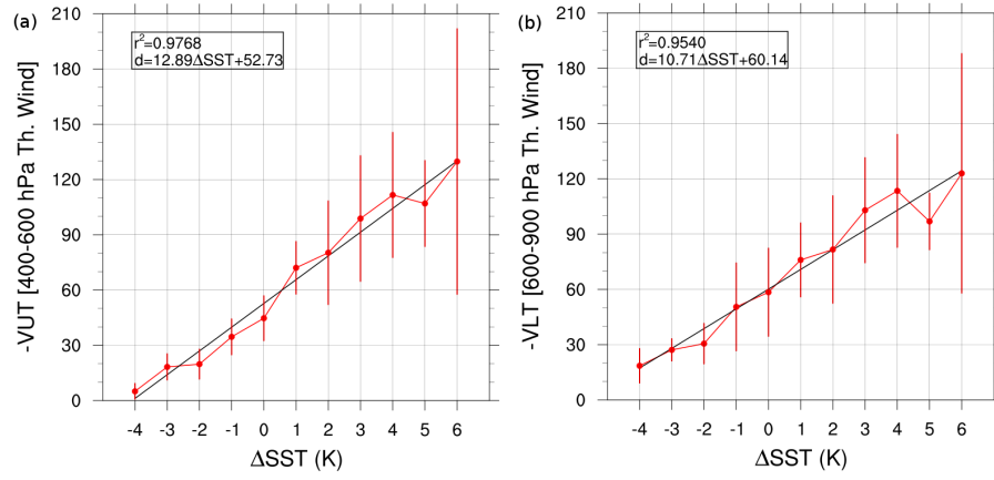
Figure 8. Dependence of composite of (a) -\text{V}_T^U and (b) -\text{V}_T^L at MWCT on SST change. The error bars represent standard deviation.
