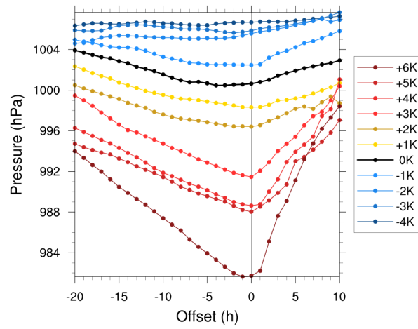
Figure 7. Composite time series of minimum pressure from -20 h before until +10 h after MWCT for each SST change.
