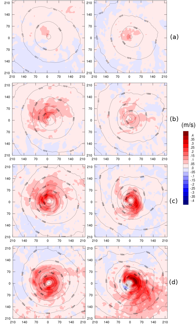
Figure 10. 10 h mean of composite vertical wind speed at 500 hPa for an SST change of a) -3 K, b) 0 K (original SSTs), c) +3 K and d) +6 K (colors) and composite mean sea level pressure (contours) between MWCT-20 h and MWCT-10 h (first column), and between MWCT-10 h and MWCT (second column). The values at the x- and y-axis indicate the distance from the center of the medicane in km.
