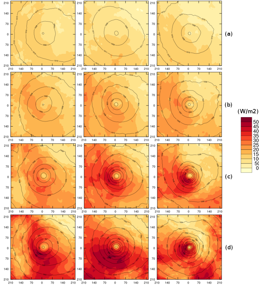
Figure 11. Composite latent heat fluxes from the sea for an SST change of a) -3 K, b) 0 K (original SSTs), c) +3 K and d) +6 K (colors) and composite mean sea level pressure (contours) at MWCT -20 h (first column), MWCT -10 h (second column) and MWCT (third column). The values at the x- and y-axis indicate the distance from the center of the medicane in km.
