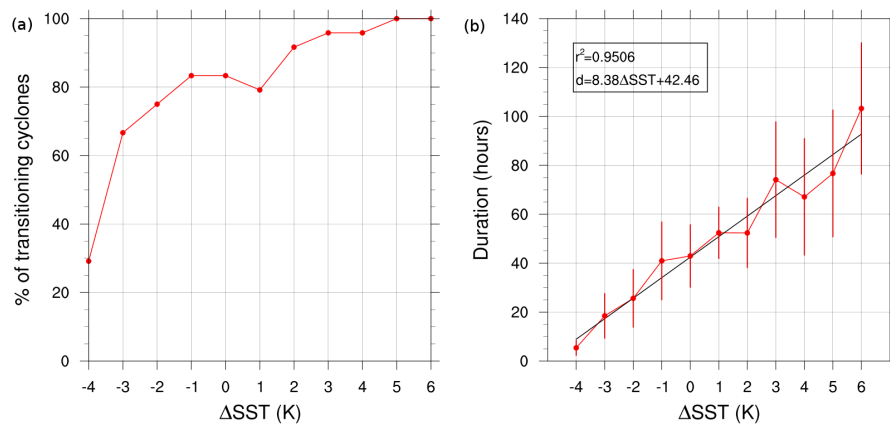
Figure 2. (a) Percentage of cyclones encountering a tropical transition over the 24-member ensembles for different SST changes, using classification criteria based on the cyclone phase space. (b) Mean period of time during which transitioning cyclones are classified as medicanes for different SST changes. Error bars represent standard deviation. The black line is based on a linear regression.
