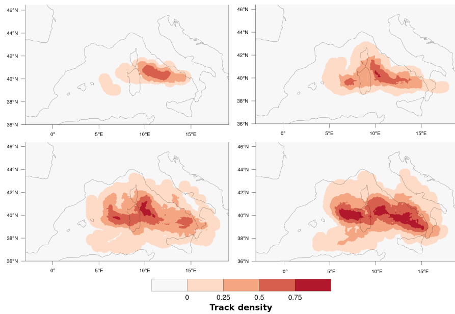
Figure 4. Track densities based on all cyclones classified as medicanes for an SST change of a) -3 K, b) 0 K (original SSTs), c) +3 K and d) +6 K.
