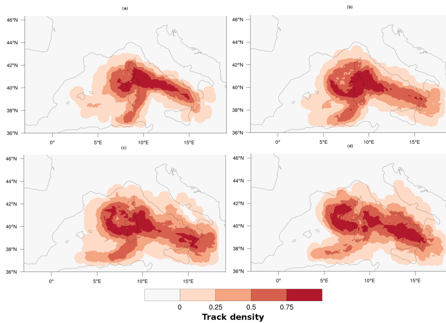
Figure 3. Track densities based on all cyclones for an SST change of a) -3 K, b) 0 K (original SSTs), c) +3 K and d) +6 K.
