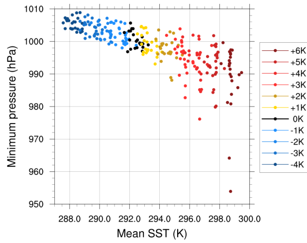
Figure 6. Dependence of minimum pressure on mean SST in a radius of 150 km, as encountered by the cyclone from from -20 h before MWCT until MWCT. Colors represent global SST change. Note that this plot is based on all cyclones and is not a composite average.
