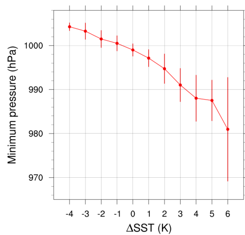
Figure 5. Dependence of composite minimum pressure on SST change. The error bars represent standard deviation.
