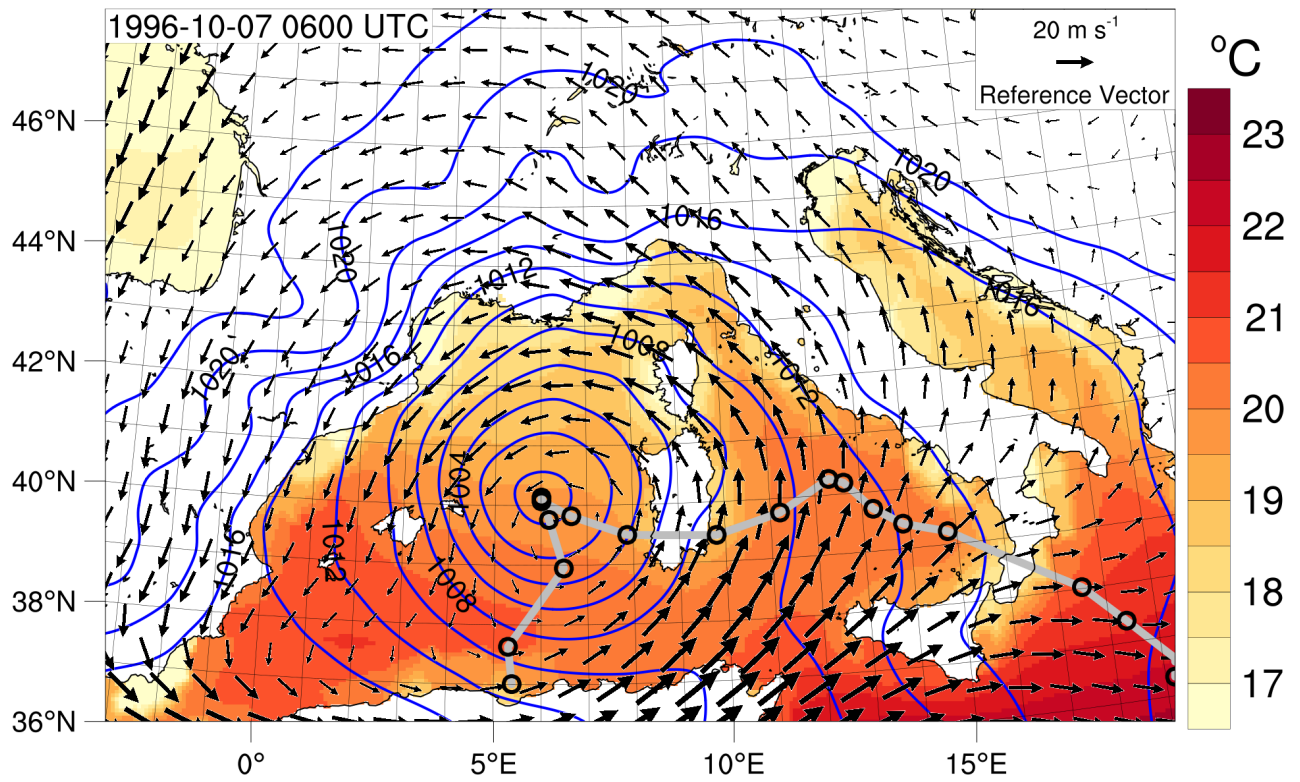
Figure 1. Inner simulation domain ( 0.0625^\circ resolution) and medicane in reanalysis. SSTs (shading), sea-level pressure (hPa, blue contours) and 500-hPa wind vectors, representative of the steering flow, are shown for the 7 th of October 1996 at 0600 UTC. The cyclone's track is shown with a grey line, marked at 6-hour intervals from 6 th October 1996 at 0600 UTC. Plot based on ERA-Interim data.
