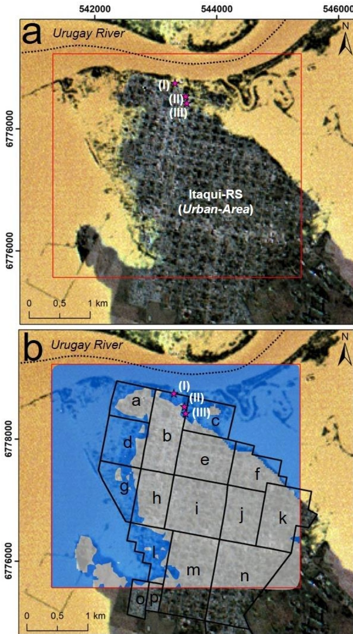
5 Figure 10: The 2017 historical flooding of the Uruguay River basin: (a) CBERS-4/MUX satellite image showing the extent of the floods on the Itaquí city area on the 12 of June 2017 (hybrid colour composition: RGBI-765NDWI); and (b) Flood simulated event in the Itaquí city for the same satellite imaging date. Neighborhoods: a) Cerrinho Dois Umbus; b) Centro; c) Ponte Seca; d) Varzea; e) Cidade Alta; f) Cohab; g) Enio Sayago; h) Estacao; i) Capelinha; j) Dr. Ayub; k) Jose da Luz; l) Vinte e Quatro de Maio; m) Chacara; n) Cafifas; o) Vila Nova; and p) Uniao. Photographic records: (I) Federal Revenue Customs Building; (II) Osvaldo Aranha street (Silva, 2017); (III) Borges do Canto street (Silva, 2017).
