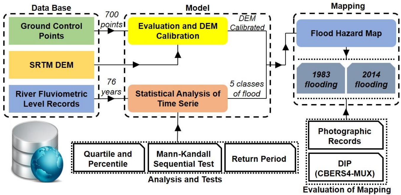
10 Figure 4: Flowchart of the proposed approach for delimitation of flood hazard mapping.
