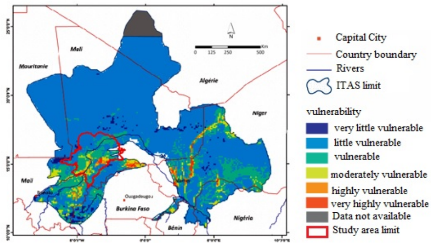
Figure 11 Vulnerability of groundwater related to climate change in the Iullemeden-Taoudeni / Tanezrouft aquifer system (ITAS) (Sahara and Sahel Observatory 2013)
