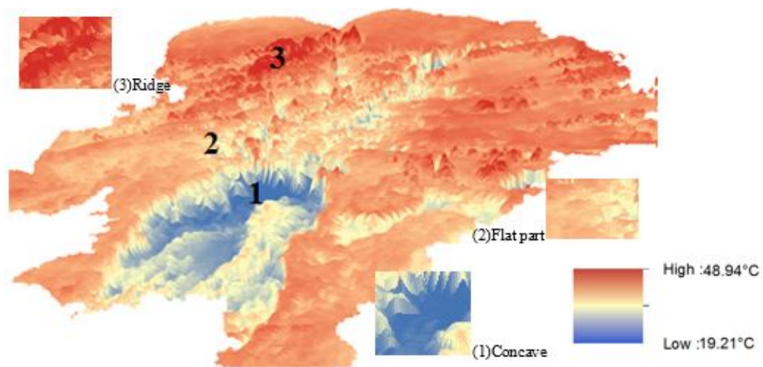
Figure 6. Modelling of the mean LST
