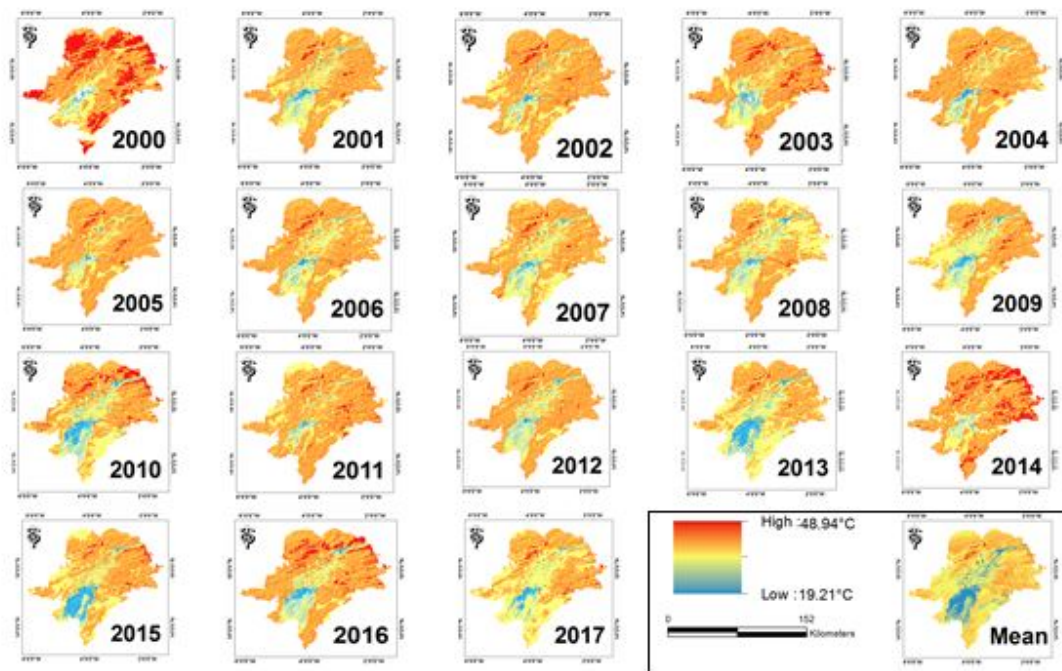
Figure 3. Land Surface Temperature (LST) change from 2000 to 2017
