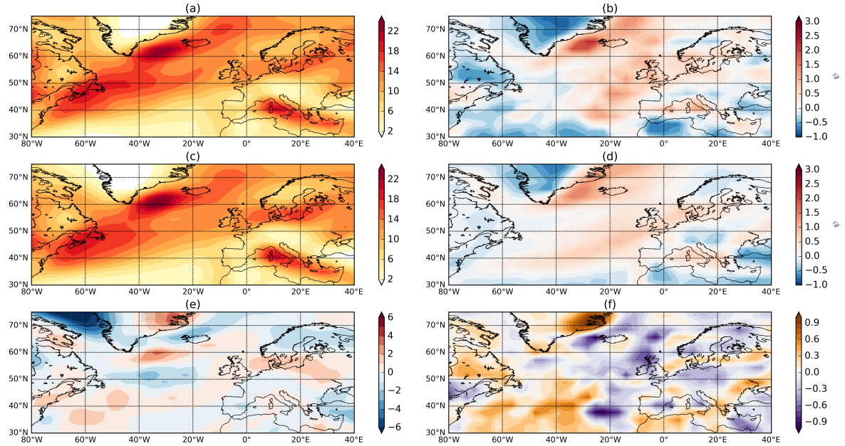
Figure 1. Track density (a) and associated dispersion (b) for ERA-Interim DJF storm track. (c), (d) same as (a), (b) but for HiGEM. (e) is the difference in track density (HiGEM-ERA-Interim), stippling indicates where the two datasets are different at the 95% level. (f) is the difference in dispersion (HiGEM-ERA-Interim). Units for (a), (c), and (e) are cyclones per month per 5° spherical cap.
