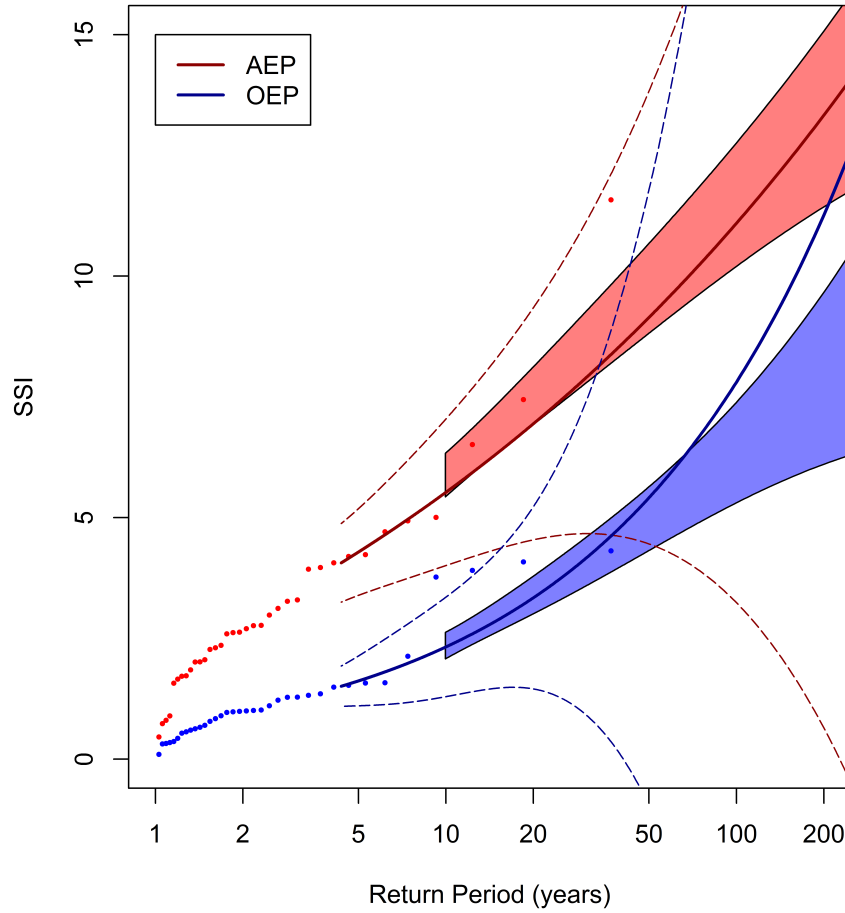
Figure A2. Return periods of the AEP (red points) and OEP (blue points) of ERA-Interim. The solid red and blue lines are GPD fits applied to the AEP and OEP using an 70th percentile threshold. The dashed red and blue regions are the associated 95% confidence intervals. The shaded red and blue regions are the 95% confidence intervals of the HiGEM_bc AEP and OEP GPD fits. The OEP and AEP are sorted independently for both ERA-Interim and HiGEM. The GPD fits and confidence intervals are only plotted only above the GPD threshold of the 90th percentile.
