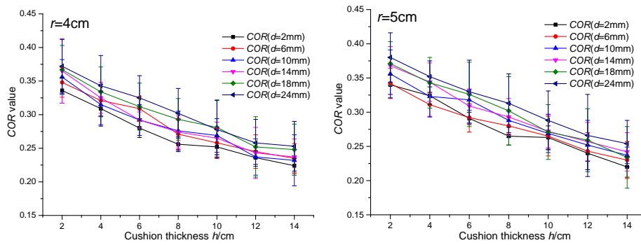
Fig.6 Comparison of the COR of blocks of different radii released from a height of 1.2m
