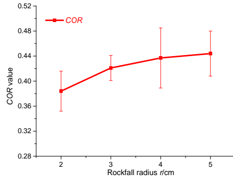
Fig. 5 The COR (Mean \pm SD) of block collisions with the plate. (Error bars: one standard deviation) COR s derived from experiments where rocks of different radii were released from a 1.2 m movement height to collide with a plate paved with cushions of different thicknesses and particle sizes are plotted in Table 2 and Figure 6. In Figure 6, mean values with error bars are shown for each test.
