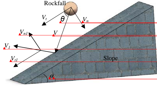
Fig.1 Motion model of rockfall
