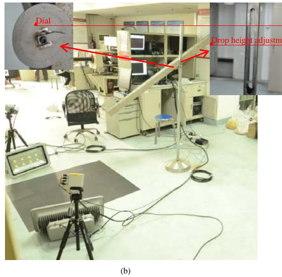
Fig.3 The experimental apparatus. (a) Model, (b) Laboratory
