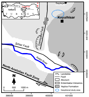
Figure 1. Geological map of study area. Arranged from Sendir and Yilmaz (2002) and Hastaoglu (2016).
