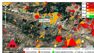
Figure 9. Seismic activity of the study area and its surroundings by the data between 1900-2015 and the landslide areas (UIDM, 2016; MTA, 2018).
