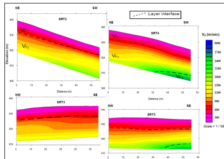
Figure 6. The seismic profiles of the area A. The uppermost boundary of the V p2 layer is the depth of the sliding surface (This depth changes between ~3-7 m). The lower velocity V p1 layer consists of soil and alluvium (the average seismic V p1 < 650 m/sec).
