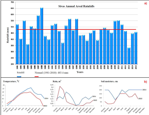
Figure 3. a) Precipitation distribution in between 1981-2015 years of Sivas (MGM, 2016). b) Graphics of monthly average temperature (T, °C), rainfall (m³) and soil moisture content (cm) of the study area and its surroundings in the years of 2013 and 2014. They were prepared from the project data (Hastaoglu et al., 2015).
