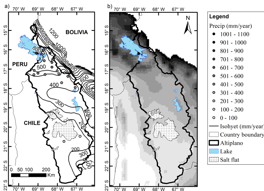
Fig. 1. R1. Map of mean annual precipitation (July 1981- June 2016) of (a) gauged data* and isohyets** and (b) CHIRPS satellite product. Source: *SENAMHI, **Ministry of Rural Development and Land of Bolivia.
