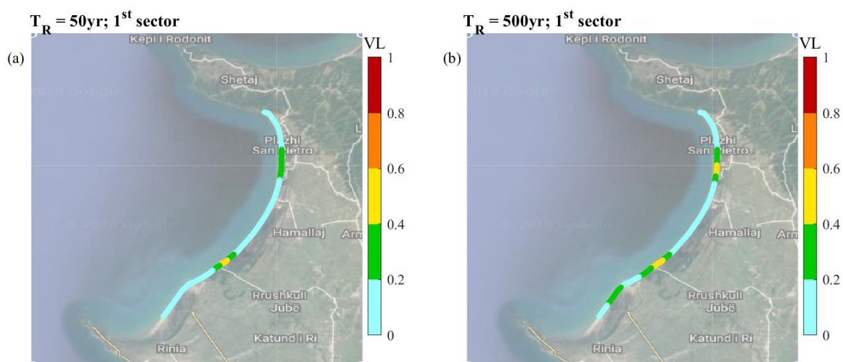
Figure 8. Run-up vulnerability levels for the Lalzit bay, using near-shore data for the 180-270 ^{\circ} N sector: a) 50yr return period; b) 500yr return period
