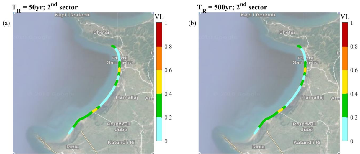
Figure 9. Run-up vulnerability levels for the Lalzit bay, using near-shore data for the 270-360°N sector: a) 50yr return period; b) 500yr return period
