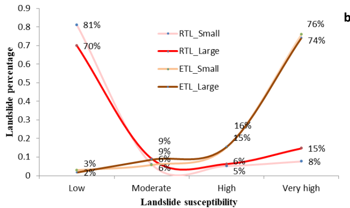
Fig. 11 Cross validation of the landslide susceptibility maps. (a) The percentage of landslides in the various classes of the RTL susceptibility map; (b) The percentage of landslides in the various classes of the ETL susceptibility map.
