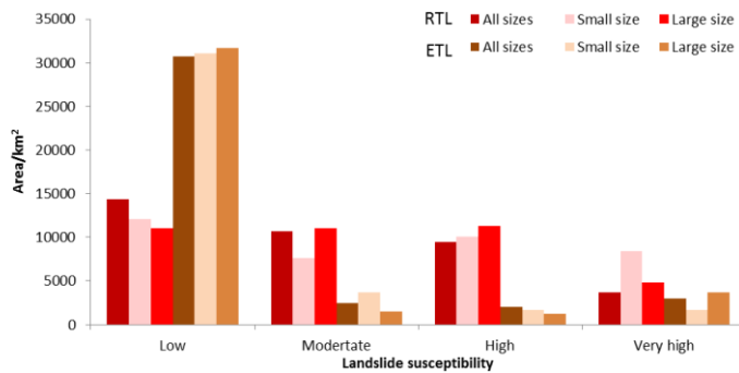
Fig. 10 Coverage of different landslide susceptibility classes for ETL and RTL maps
