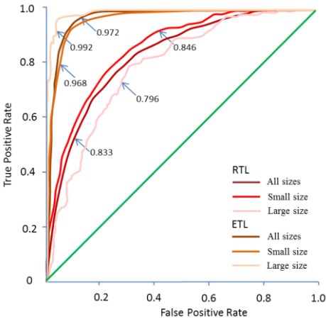
Fig. 8 ROC curves for the susceptibility assessing models to different sizes of RTL and ETL
