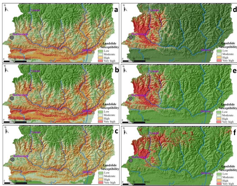
Fig. 9 Susceptibility maps for different sizes of RTL and ETL: (a) for all RTLs; (b) for small RTLs; (c) for large RTLs; (d) for all ETLs; (e) for small ETLs; (f) for large ETLs.
