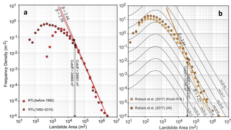
Fig. 5 Landslide frequency - area distributions of (a) RTL inventories, (b) ETL inventories created for Koshi River basin and ETL inventories created for the entire landslide-affected area of the 2015 Gorkha, Nepal earthquake (Roback's landslide inventory was validated). Cutoff and \beta values are calculated using the method proposed by Clauset et al. (2009).
