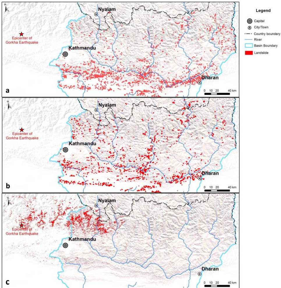
Fig. 4 Landslide inventories of the Koshi River basin (a) Rainfall induced landslide inventory of events before 1992; (b) Rainfall induced landslide inventory for the period between 1992 to 2015; (c) Inventory of landslides triggered by the 2015 Gorkha earthquake (Roback et al. 2017).
