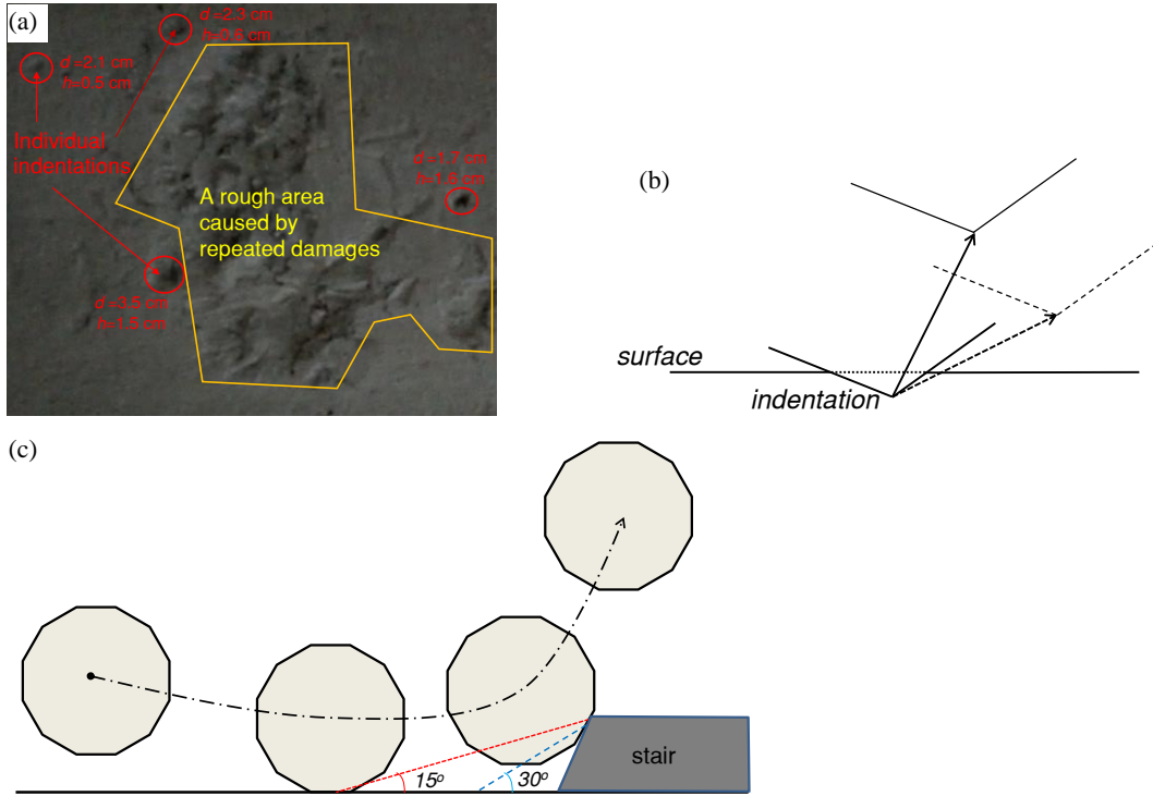
Figure 12. (a) Individual indentations and a rough area caused by the impacts and their influence on the rebound motion: (b) a simplified configuration used to evaluate the effect of the indentation; (c) a small stair model used to evaluate the effect of the macro roughness
