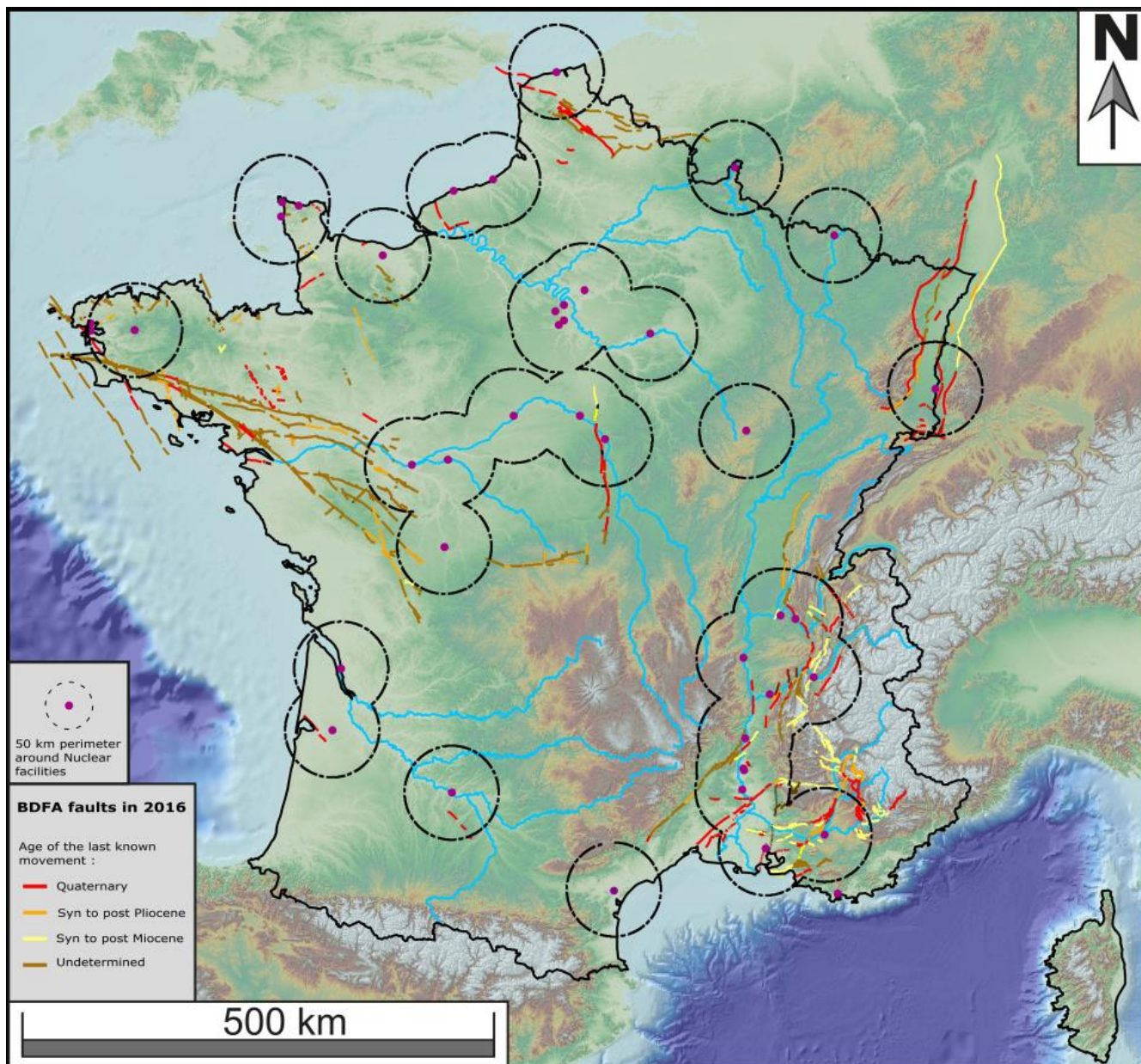
Figure 1: Map of BDFA ( Google earth kml file provided in annexes ) at the scale of metropolitan France. Faults coloured by the age of the last known movements. Black circles represent a 50km perimeter around each nuclear facility.
