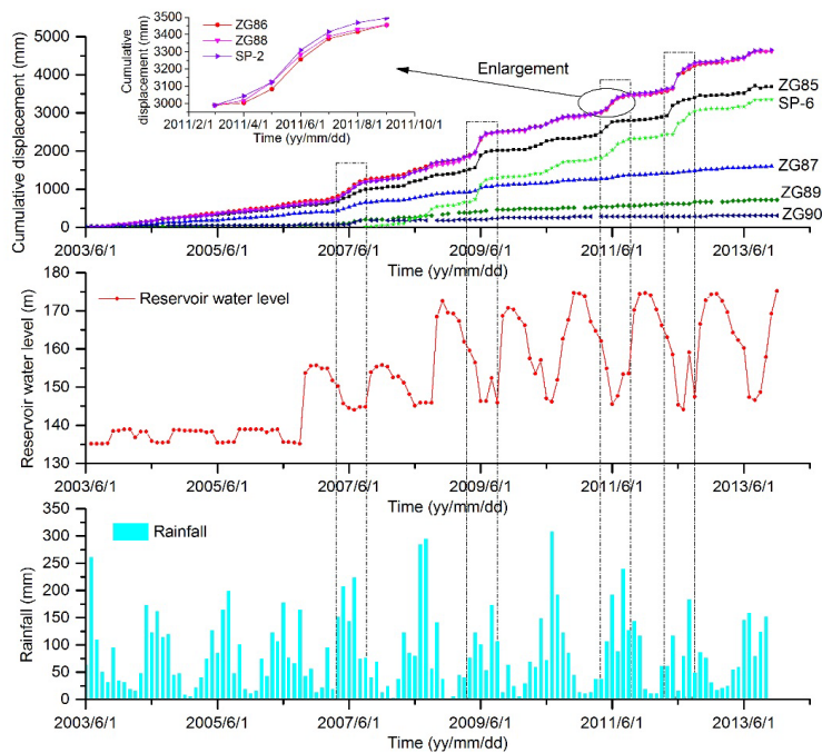
1 2 Fig. 6 The relationships between rainfall, reservoir water level and displacement
