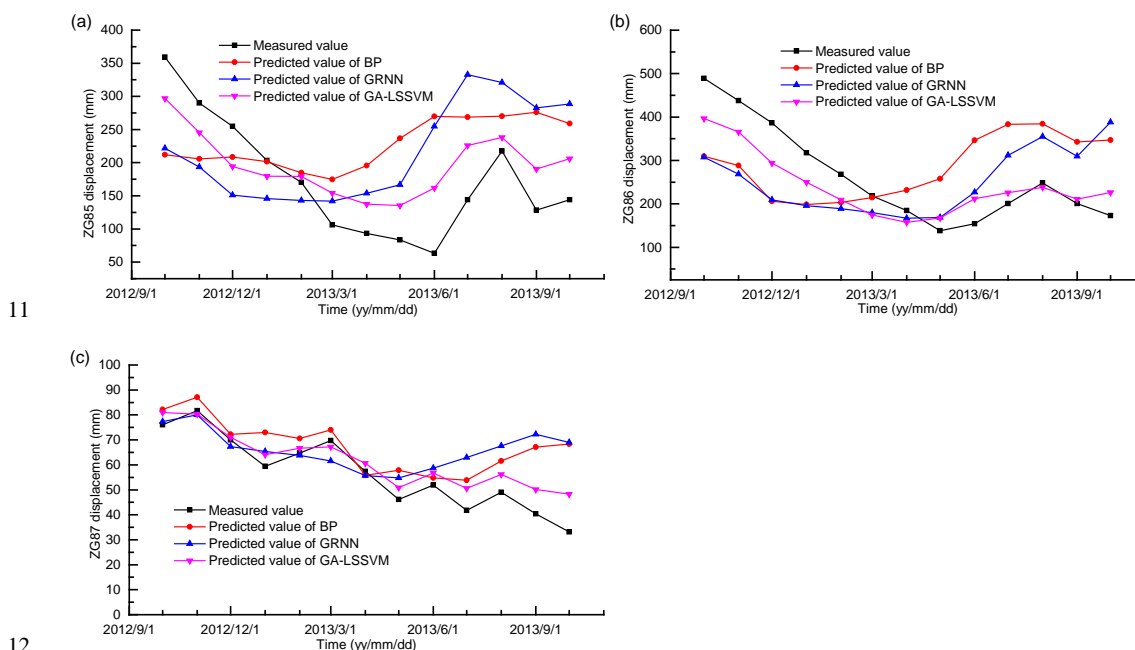
11 12 Fig. 12 Measured displacement and predicted periodic displacement of Shuping landslide
