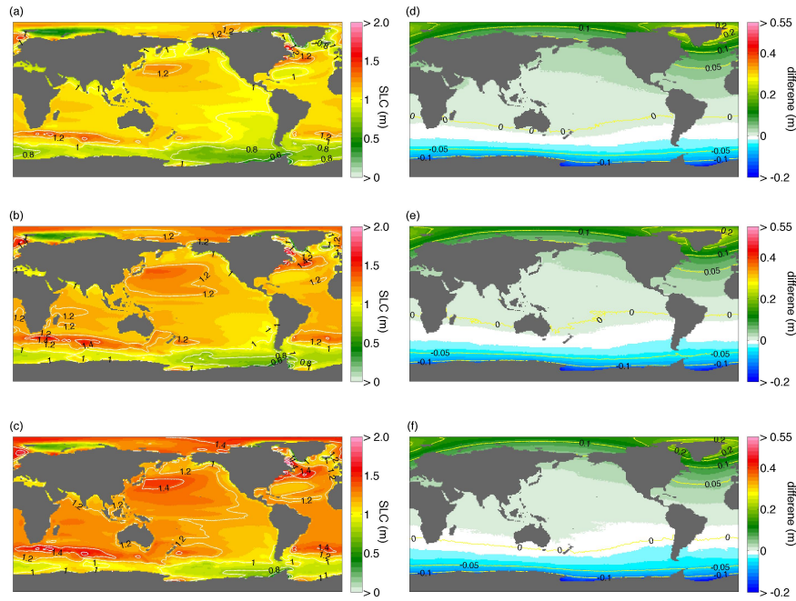
Figure 8. Left column: a. 90 th , b. 95 th and c. 97.5 th percentile for the asymmetric Ritz-distribution of dynamical ice sheet mass loss of East and West-Antarctica ice sheets (EAIS and WAIS) combined with symmetric IPCC-based contributions of dynamical ice mass loss of the Greenland ice sheet (GIS) and regional SLC projections following RCP8.5 (Slangen et al., 2014). Right column: difference between d. 90 th , e. 95 th and f. 97.5 th percentile for asymmetric Ritz and symmetric IPCC-based ice dynamical contribution of EAIS and WAIS, both combined with symmetric IPCC-based contributions of dynamical ice mass loss of the Greenland ice sheet (GIS) and regional SLC projections following RCP8.5 (Slangen et al., 2014). Percentiles for the symmetric IPCC-AR5 probability distribution are depicted in Figure SA2.
